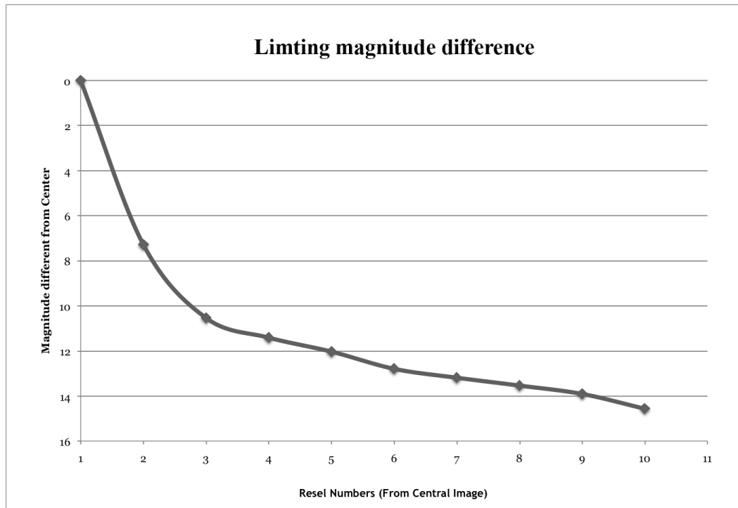
Figure 4.2: Maximum magnitude difference attainable at a given distance from the center of the PSF. (Obtained by sampling the numerically simulated PSF) similar to figure 3.10.
