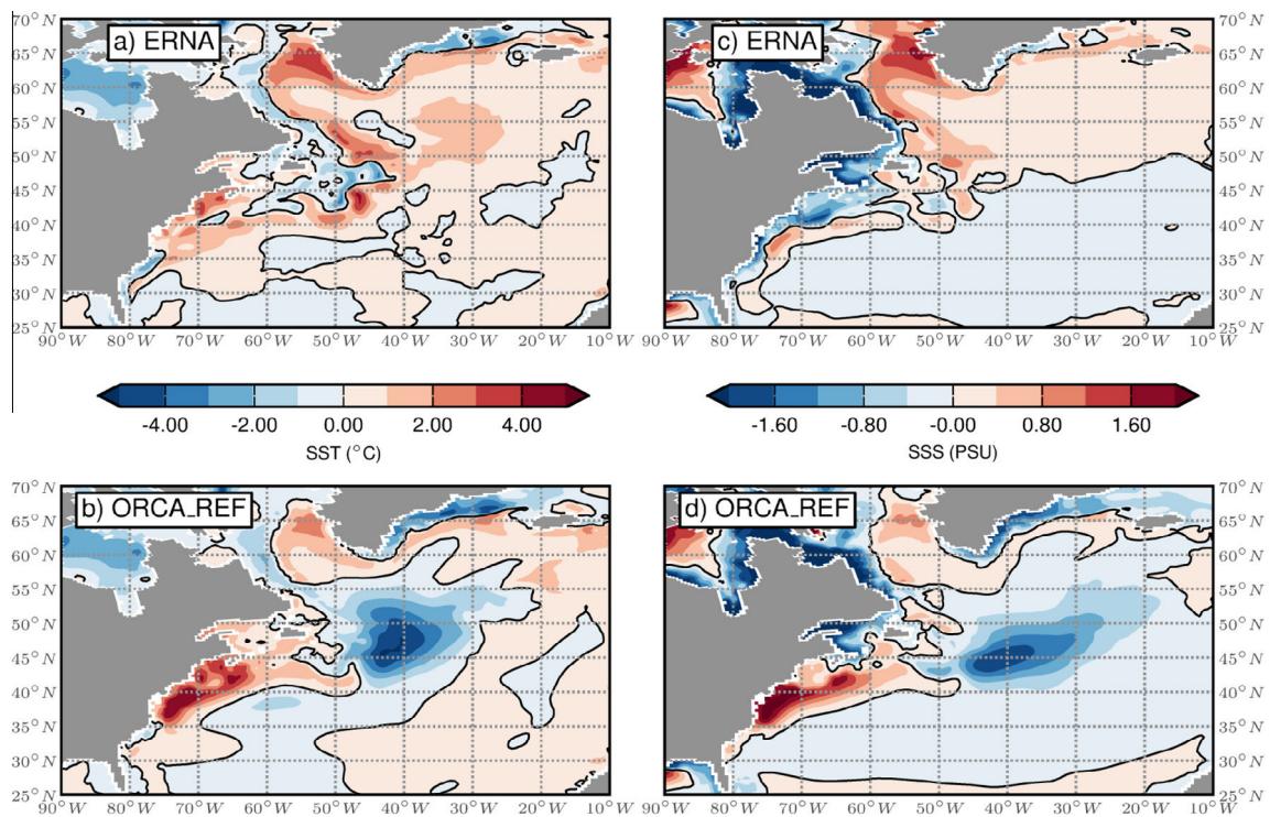
Fig. 7. Sea Surface Temperature (SST) (a,b) and Sea Surface Salinity (SSS) (c,d) anomalies to observed Levitus climatology (in °C and PSU) in ERNA (a,c) and ORCA_REF (b,d), averaged over the period 1990–2009.
