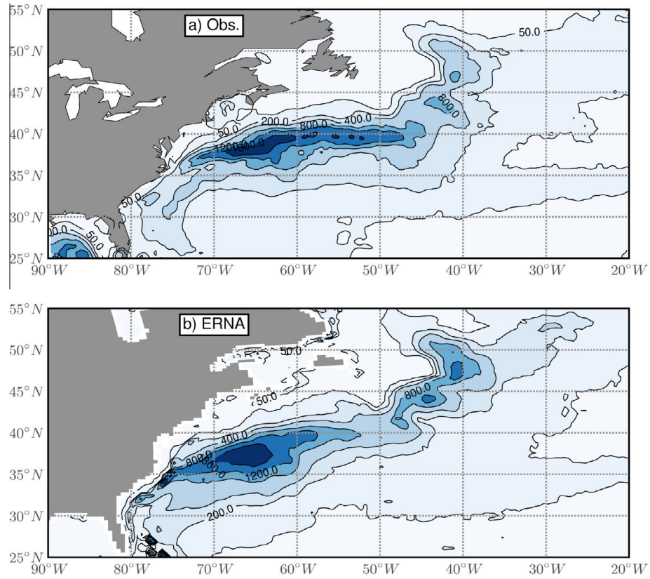
Fig. 3. Eddy Kintetic Energy (EKE) averaged over the period 1993–2009 in AVISO observations (a) and ERNA (b) in \text{cm}^2 \text{s}^{-2} .
