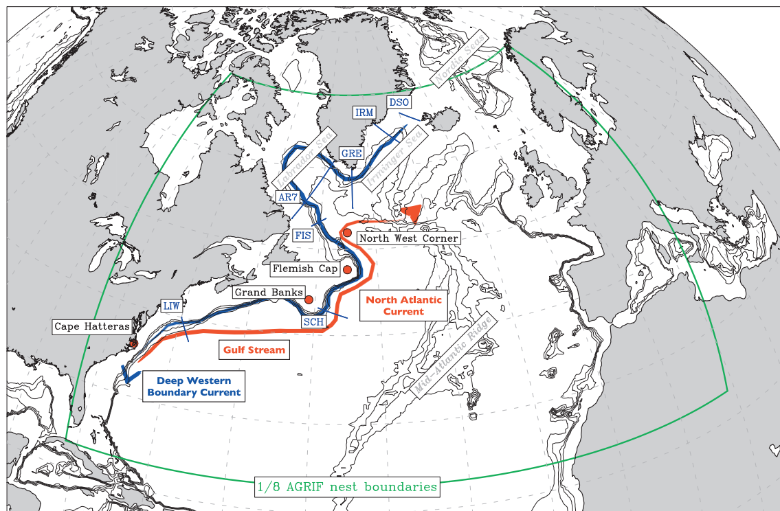
Fig. 1. Area covered by the 1/8° nest over the North Atlantic in ERNA configuration, with a schematic location of major western boundary currents at the surface (red thick line) and at depth (blue thick line). Thin blue lines represent vertical sections location; LIW refers to “LineW” (Toole et al., 2011); SCH refers to Schott et al. (2006) section at 43°N; FIS refers to Fischer et al. (2010) section at 53°N; AR7 refers to the AR7W section in the Labrador Sea (Hall et al., 2013) and the DSO section through the Denmark Strait overflow (Vage et al., 2011b). (For interpretation of the references to color in this figure legend, the reader is referred to the web version of this article.)
