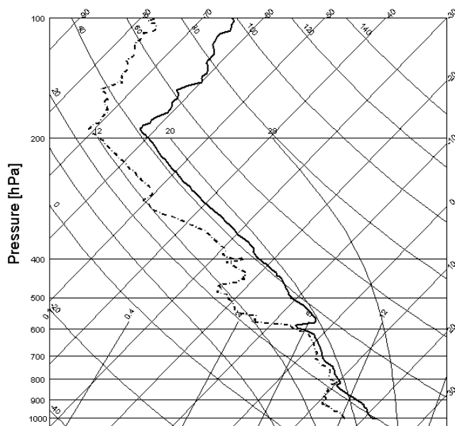
Figure 4. Skew T-log p diagram from radiosoundings launched at Milan/Linate on 25 September 1999 at 1200 UTC. Continuous and dotted lines relate to air and dew point temperature (in ^{\circ}\text{C} ) respectively.
