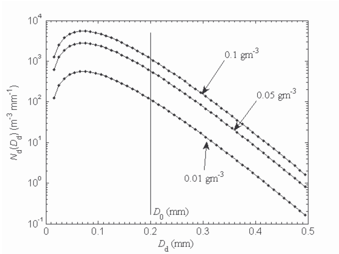
Figure 6: Drizzle drop size distribution (DDSD) for a parameter \mu equal to 2 and several maximum drizzle water content ( 0.01 , 0.05 , and 0.1 \text{ g m}^{-3} ). Median diameter is D_0 = 0.2 \text{ mm} (solid vertical line).
