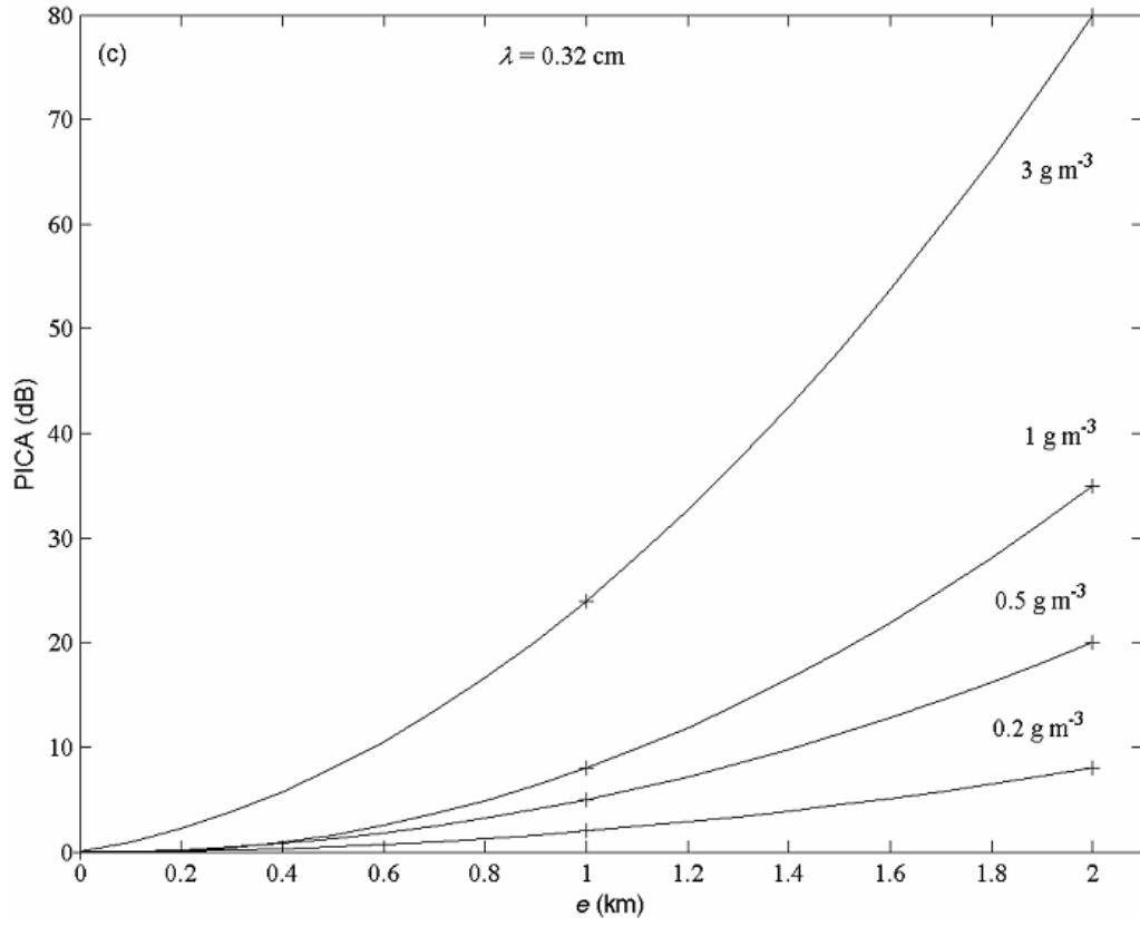
Figure 16: Maximum value of PICA (dB) with respect to cumulus thickness e (km) according to cloud maximum liquid water content ( M_c^{\max} = 3, 1, 0.5 , and 0.2 \text{ g m}^{-3} ); cloud shape factor is 5. Wavelengths of observations are 3.2 cm (a), 0.86 cm (b), and 0.32 cm (c).
