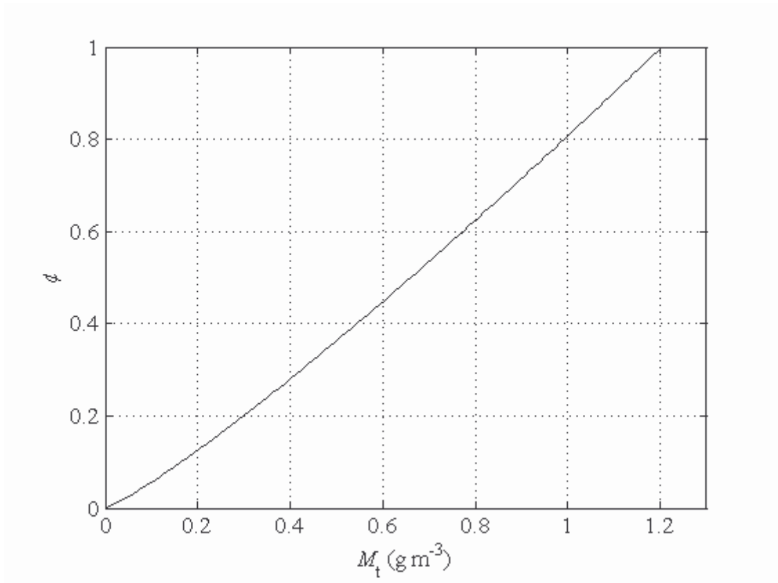
Figure 8: Dependence of the cloud liquid water content threshold M_{c, t} ( \text{g m}^{-3} ) above which drizzle drops can be expected in warm clouds (stratocumulus and cumulus) with normalized altitude \phi in cloud.
