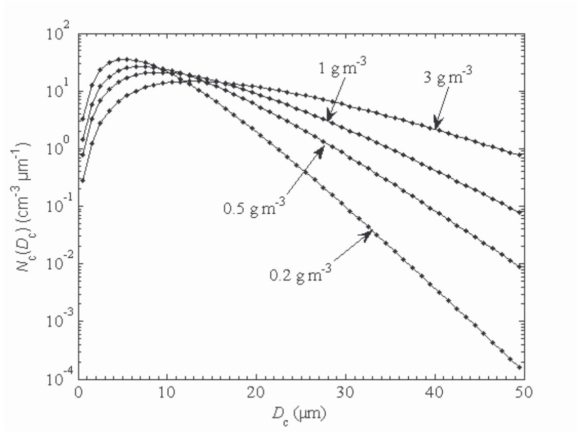
Figure 2: Cloud droplet size distribution (CDSD) represented by (7), D_c being the droplet diameter and N_c the volumic concentration per class of diameter. CDSD is displayed for four values of M_c^{\max} (0.2, 0.5, 1, and 3 \text{g m}^{-3} ) and N_t equal to 350 \text{cm}^{-3} .
