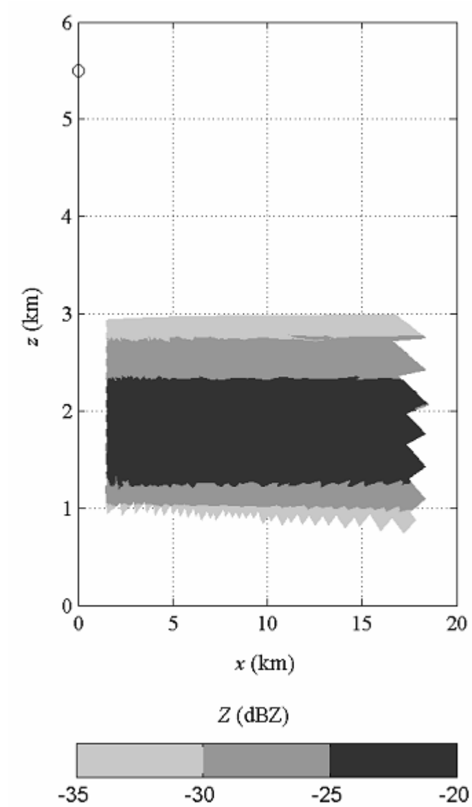
Figure 10: Simulation of the observed stratiform cloud reflectivity at the reference wavelength of 10.7 cm. The radar is represented by symbol “o” at (x, z) = (0, 5.5 \text{ km}) .
