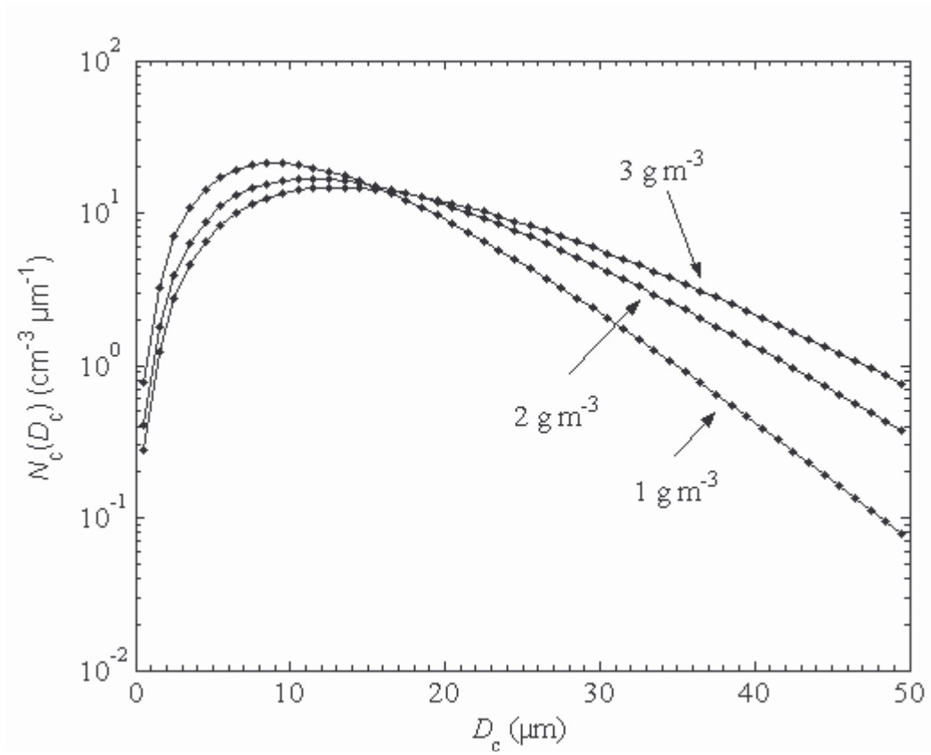
Figure 3: Cloud droplet size distribution (CDSD) represented by a Khrgian and Mazin (1952) distribution. CDSD is displayed for three values of the cloud liquid water content and for a total droplet concentration fixed at 350 \text{ cm}^{-3} . D_c is the droplet diameter and N_c the volumic concentration per diameter class.
