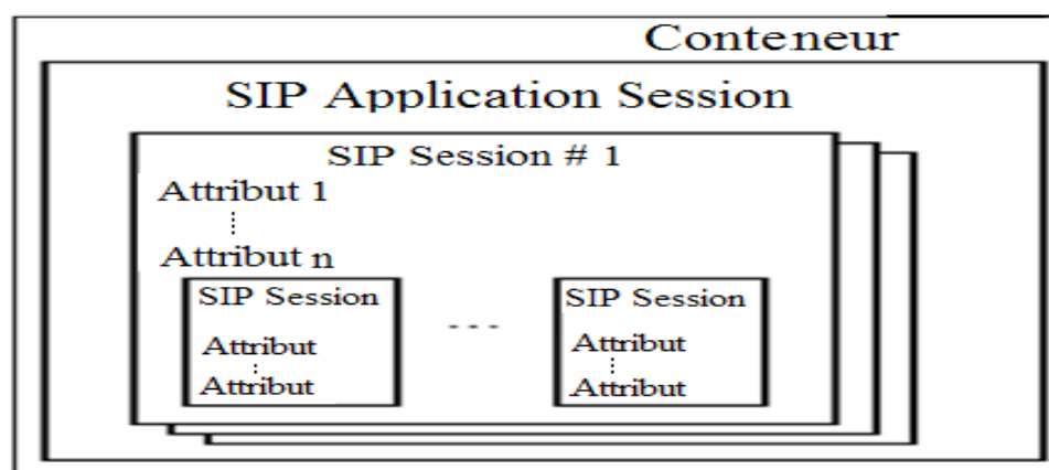
Figure 4.3 SipSession vs SipApplicationSession Tirée de (Oracle, 2011a)
