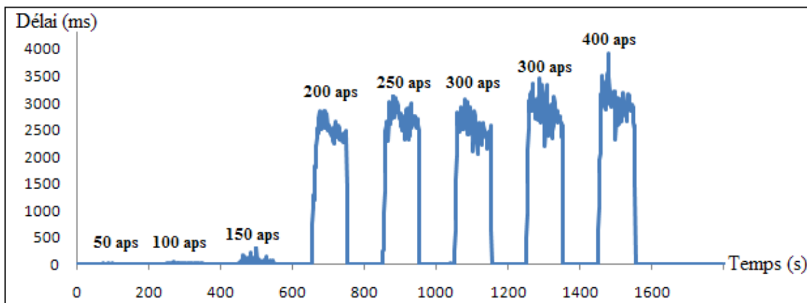
Figure 5.6 Le délai 'Invite-180'
