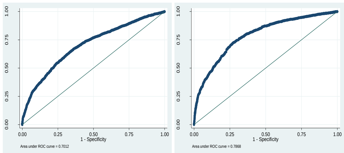
Figure 15: Post-estimation diagnostic of the model in 2001 (left) and 2007 (right): Receiver Operating Characteristic (ROC) curve
