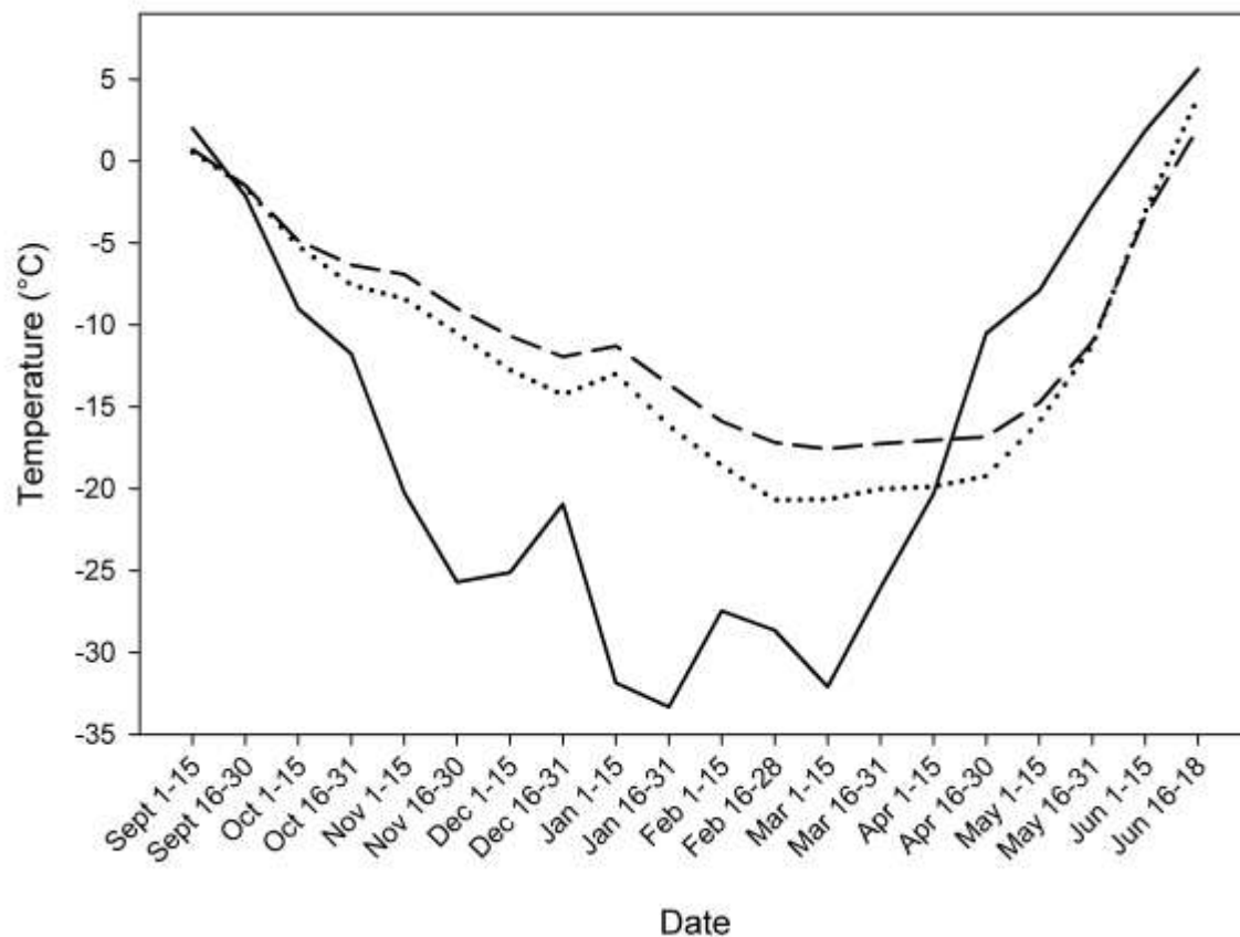
Figure S2. Mean daily temperatures (°C) for Bylot Island over winter 2010-11. Data show temperature of ambient air (solid line; from a weather station at the site), at ground-level on the control grid (dotted lines; n = 10 I-Buttons ® sensors), and at ground level in the snow-manipulated grid < 10 m from fence (dashed lines; n = 10 sensors). See also Reid et al. (2012).
