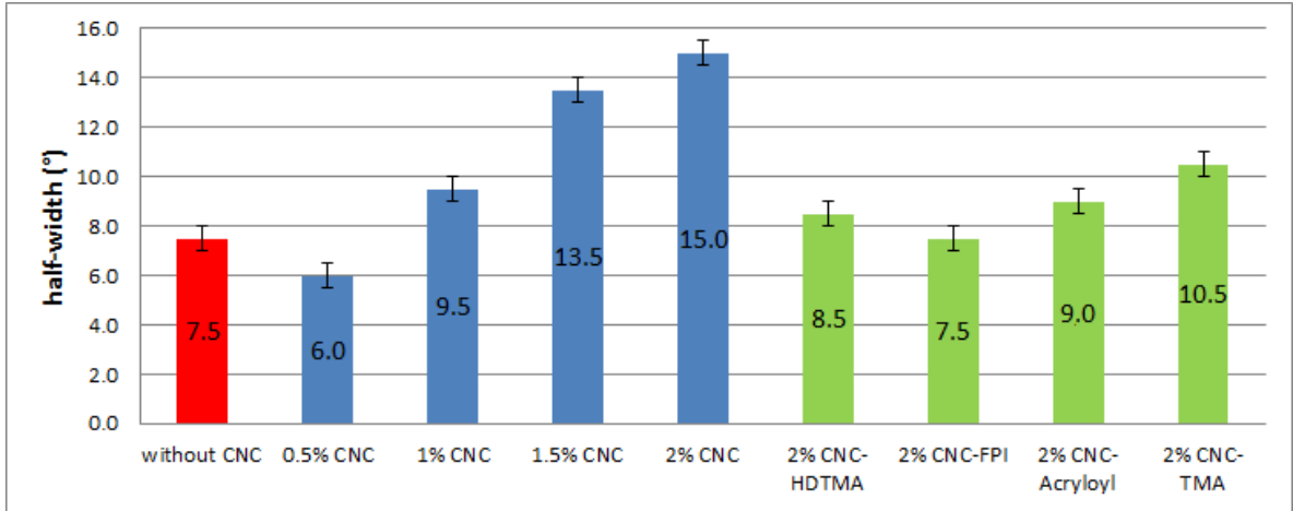
Figure 5.10. Half-width of angular spread of backscattering from varnishes without and with modified and unmodified CNCs.
