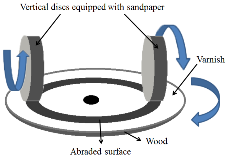
Figure 4.5. The abrasion resistance set-up using the Taber Abraser.
