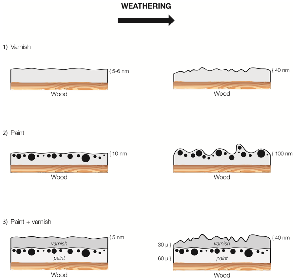
Figure 6.11. Schematic interpretation of effect of UV light weathering on surface texture, from AFM, on various varnished and painted wood surfaces (drawing not to scale as to particle size / roughness / thickness).
