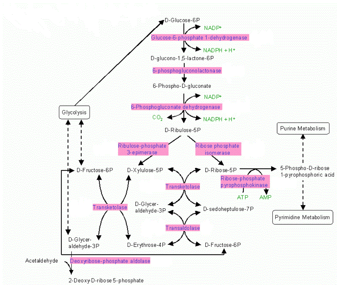
Figure 8 : Le cycle des pentoses phosphates [12].
