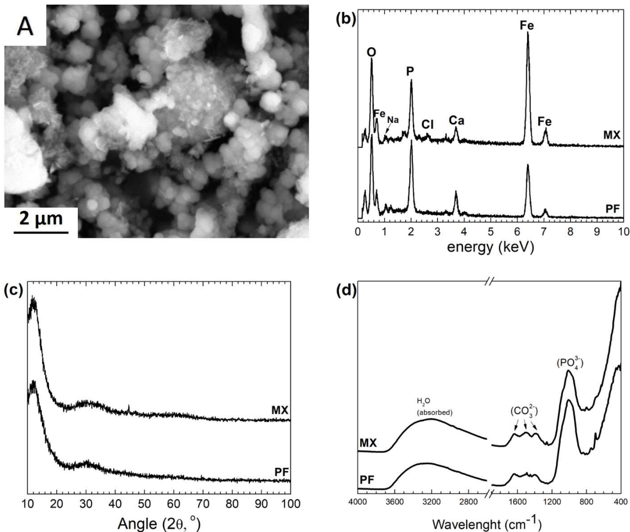
Figure 5.7. a) representative image of degradation products after 50 days of immersion of MX sample, b) EDS, c) XRD and d) FTIR on degradation precipitates after 50 days of immersion
