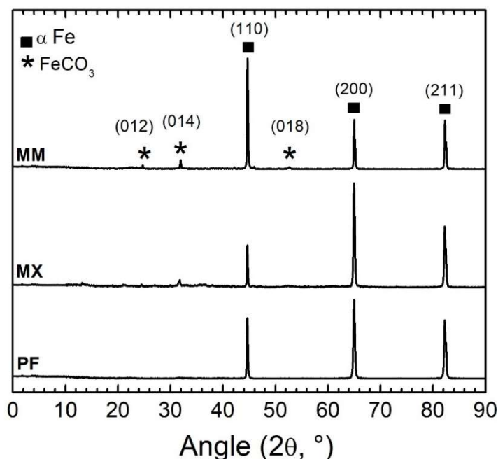
Figure 4.7. XRD patterns on the corroded surfaces after 240 hours of immersion in modified Hanks' solution for Fe and Fe/ \text{Mg}_2\text{Si} composites
