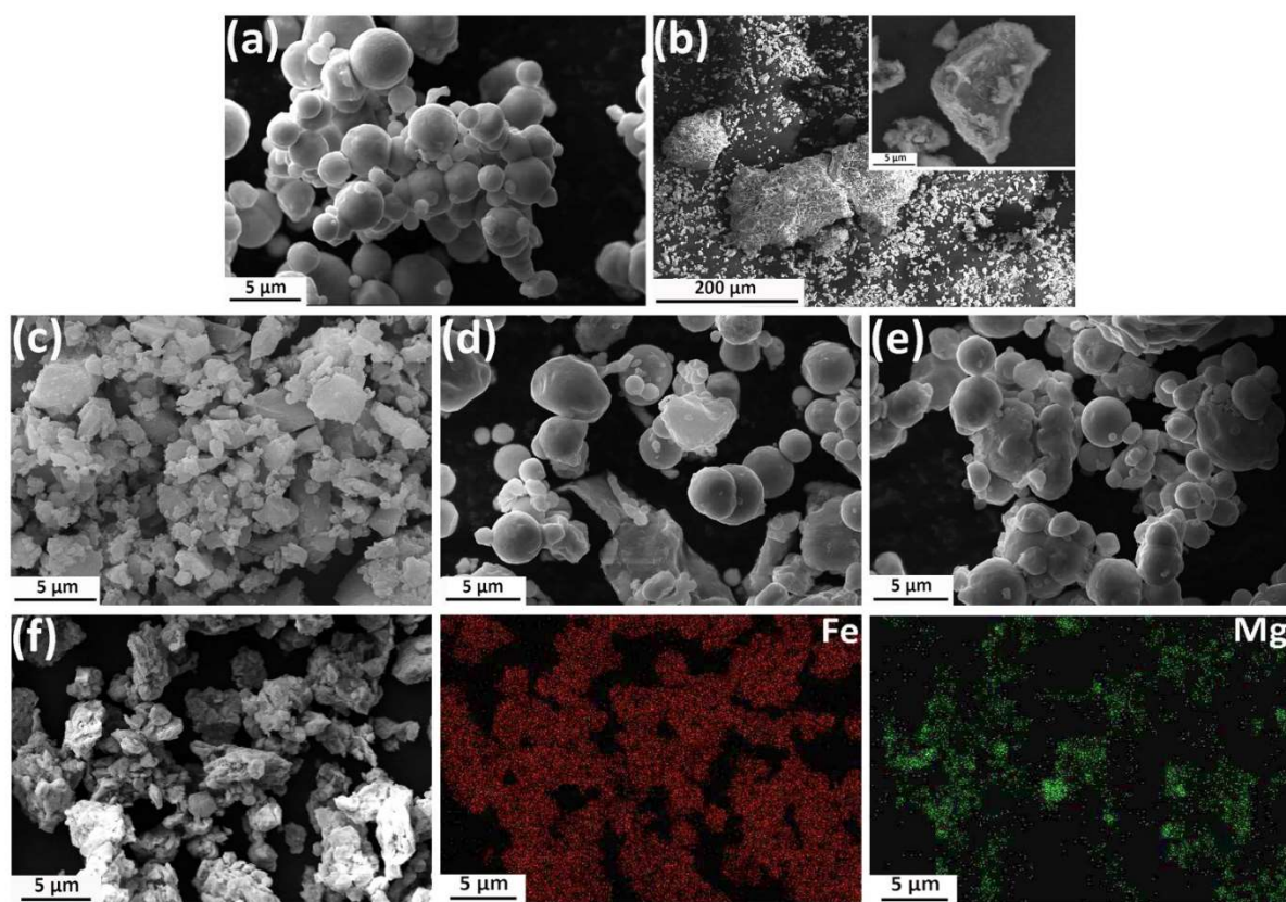
Figure 3.1. SEM morphology of the powders used in this study: a) as-received Fe powder, b) as-received \text{Mg}_2\text{Si} powder, c) high energy ball milled \text{Mg}_2\text{Si} powder, d) MX, e) BM, f) MM and its corresponding elemental maps for Fe and Mg, respectively
