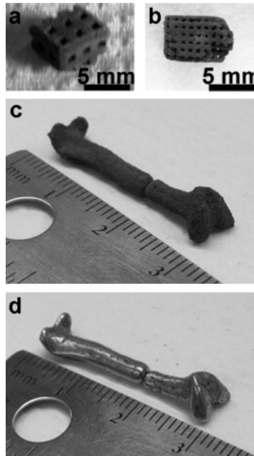
Figure 1.12. Photographs 3-D printed samples from Fe–30Mn powder after sintering: parts with square pore sizes of lengths (a) 1 mm and (b) 500 \mu\text{m} ; miniature human femur (c) before finishing and (d) after finishing [105]
