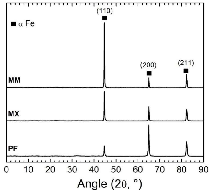
Figure 4.2. X-ray diffraction patterns of Fe and Fe/ \text{Mg}_2\text{Si} composites
