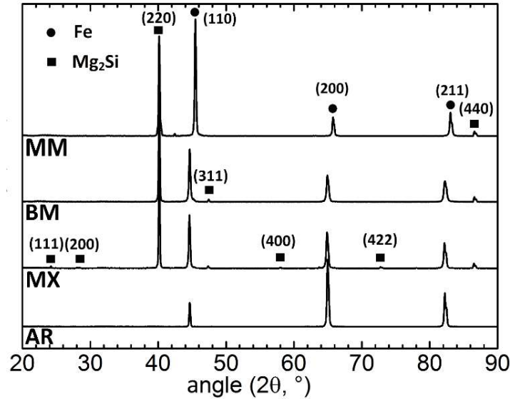
Figure 3.3. X-ray diffraction patterns of Fe and Fe/ \text{Mg}_2\text{Si} composites. Table 3.1 shows the preparation details for AR, MX, BM and MM samples, respectively
