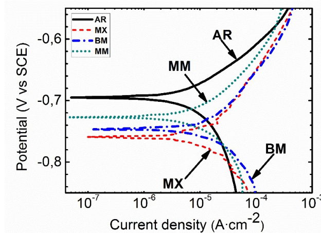
Figure 3.5. PTD curves for Fe/ \text{Mg}_2\text{Si} composites compared to the pure Fe
