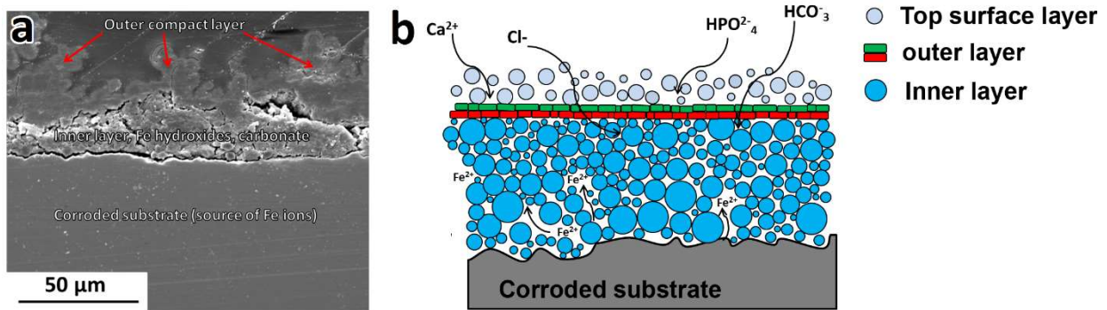
Figure 5.9. a) SEM micrograph of PF100 cross-section showing the layered structure of protective films formed during degradation b) schematic showing characteristic features of the degradation deposit
