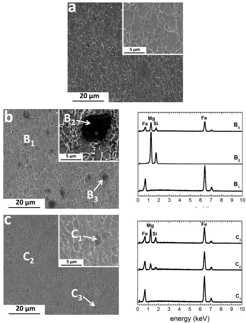
Figure 4.1. SEM micrographs of powder metallurgy Fe, Fe/Mg 2 Si composites and corresponding EDS spectra a) PF, b) MX, c) MM
