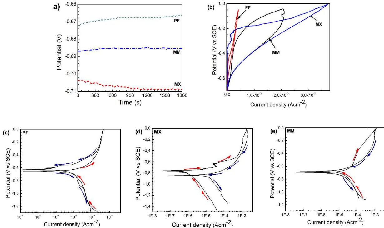
Figure 4.3. Electrochemical measurement plots for Fe/ \text{Mg}_2\text{Si} composites compared to pure Fe a) OCP, b) hysteresis loop, and cyclic polarization curves for c) PF, d) MX, and e) MM samples
