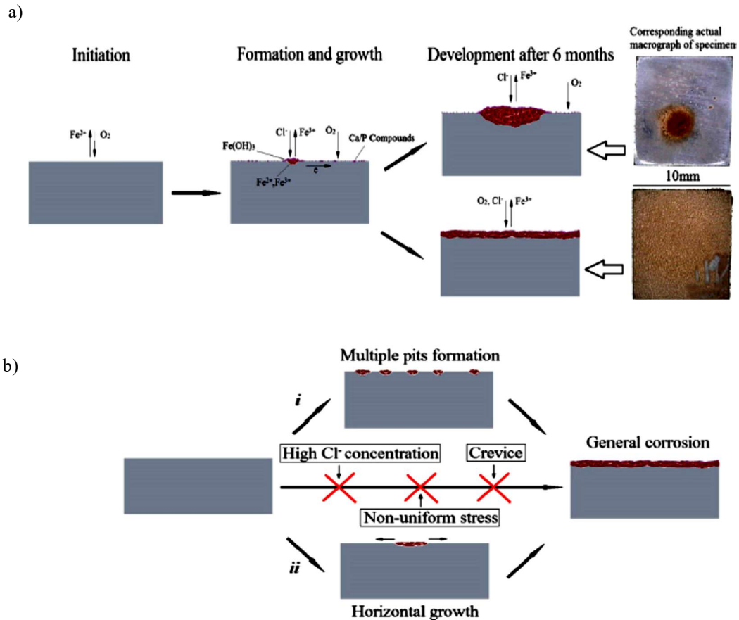
Figure 1.13. Schematic diagram illustrating a) corrosion mechanism of Fe-based BM in Hanks' solution, b) ideal corrosion process of Fe-based BM [80]
