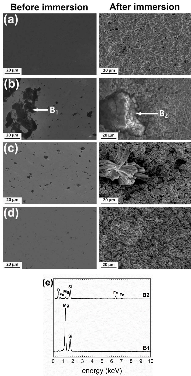
Figure 3.6. (a) to (d). SEM images of samples' surface morphology before and after static immersion test in Hanks' solution for 14 days a) AR, b) MX, c) BM, d) MM, (e). EDS analyses related to points B 1 and B 2 of Fig. 3.6 (b).
