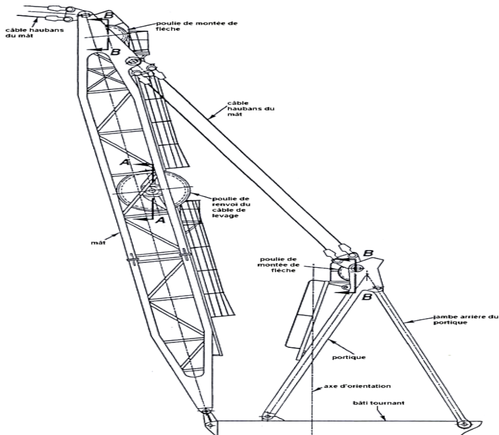
Figure 18 : le mât
