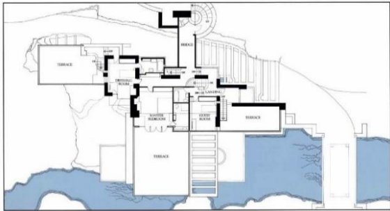
Figure 62 : Plan_Fallingwater [Ka21].
