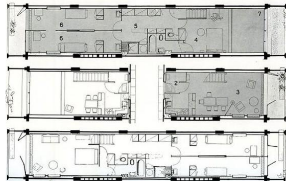
Figure 84 : Plan_La Cité Radieuse [Pin21].
