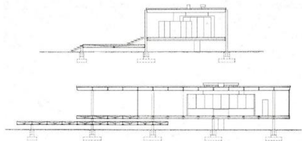
Figure 71 : Coupes_Farnsworth House [DAD15].
