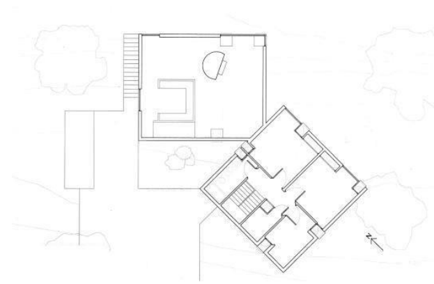
Figure 72 : Plan_Fisher House [Gal21].
