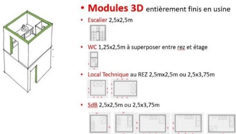
Figure 105 : Schéma_Ncube_Naturhome.
