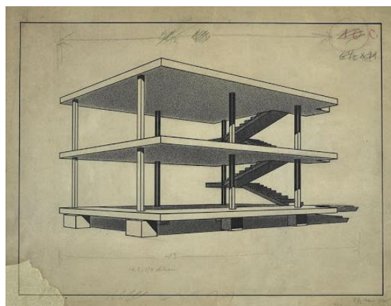
Figure 44 : Maison Dom-ino_Le Corbusier_1914 [Fon21].
