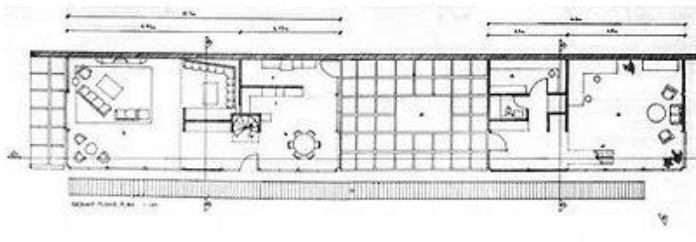
Figure 65 : Plan_Eames House [Min21].
