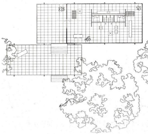
Figure 69 : Plan_Farnsworth house [DAD15].
