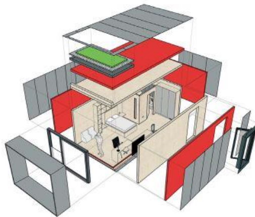
Figure 101 : Axonométrie_ Student Village [Wil20].
