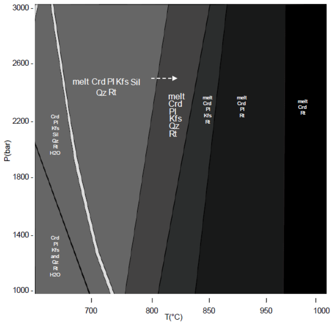
Figure 3.10: NCKFMASHMT P-T pseudosection for Bedded Pyrrhotite Unit (BPU) sample A4-18-09 from the contact aureole (Virginia Formation). Field of melt-Crd-Pl-Kfs-Qz-Rt at ~800°C and 2.5 kbars is the most consistent with the mineral assemblage in the sample A4-18-09 (white arrow). Abbreviations used for pseudosections (Whitney and Evans, 2010): Bt = Biotite; Crd = Cordierite; Hc = Hercynite; Ilm = Ilmenite; Kfs = K-feldspar; Pl = Plagioclase; Qz = Quartz; Rt = Rutile; Sil = Sillimanite.
