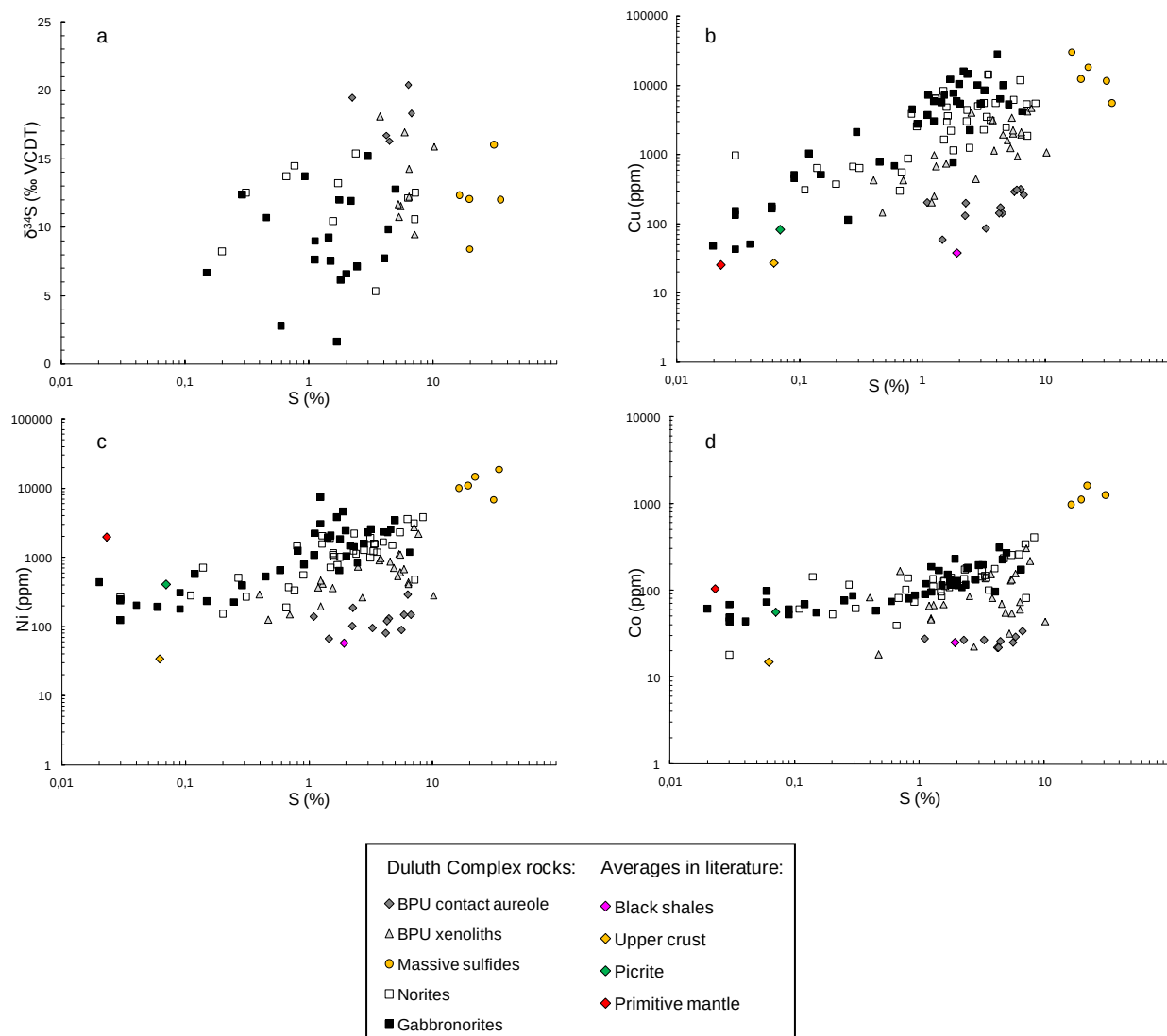
Figure 2.4: Plots of (a) \delta^{34}\text{S} , (b) Cu, (c) Ni and (d) Co vs. S. Isotopic ratio \delta^{34}\text{S} of mantle is comprised between 0 and 1‰. Averages of black shales, upper crust, picrites, and primitive mantle are shown for reference (Dionne-Foster, 2007; Lyubetskaya and Korenaga, 2007; Hu and Gao, 2008; Henrique-Pinto et al., in press). Abbreviation:
