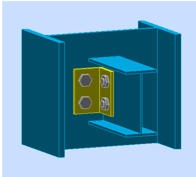
Figure VII.4 Assemblage poteau-poutre secondaire.
