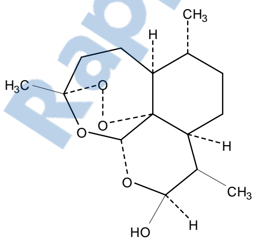
DIHYDROARTEMISININ
