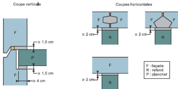
Figure I-1: joints de mortier continus
