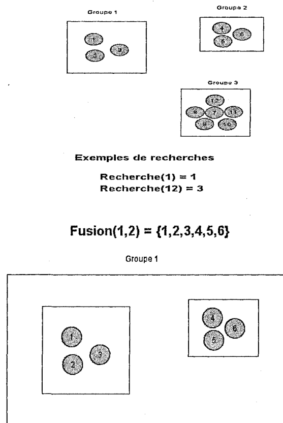
Figure 1 : Ensembles disjoints
