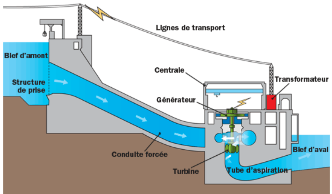
Figure I.2 centrale hydraulique
