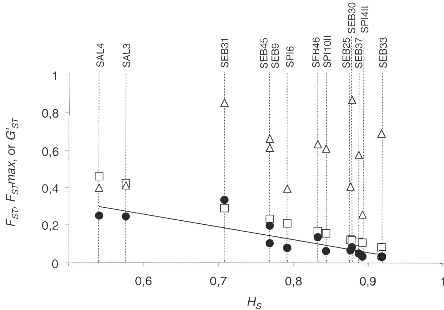
Figure 3.4 Graph showing the relationship between the locus polymorphism (represented by H_s , i.e. the mean within-sample observed heterozygosity), and the indices of differentiation F_{ST} (●), and G'_{ST} (△). F_{STmax} (□) is the theoretical maximal single-locus F_{ST} value, computed as 1 - H_s . The correlation (black line) between F_{ST} and H_s is significant, according to a Spearman rank test ( r_s = -0.92 ; P < 0.0001 ).
