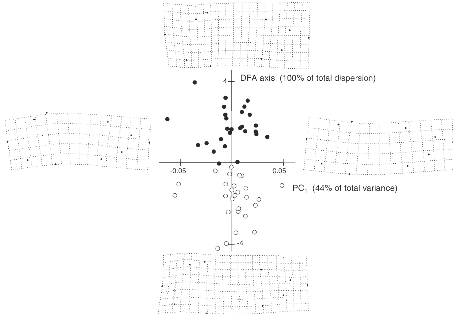
Figure 2.3 PC 1 scores (with % of total variance) versus DFA scores (with % of total dispersion) for the fresh–thawed comparison study. Deformation grids show shape changes associated with PC 1 (i.e., the upward/downward arching) and shape changes (magnified 3 times) between freshly caught (O) and thawed (●) specimens along the discriminant axis.
