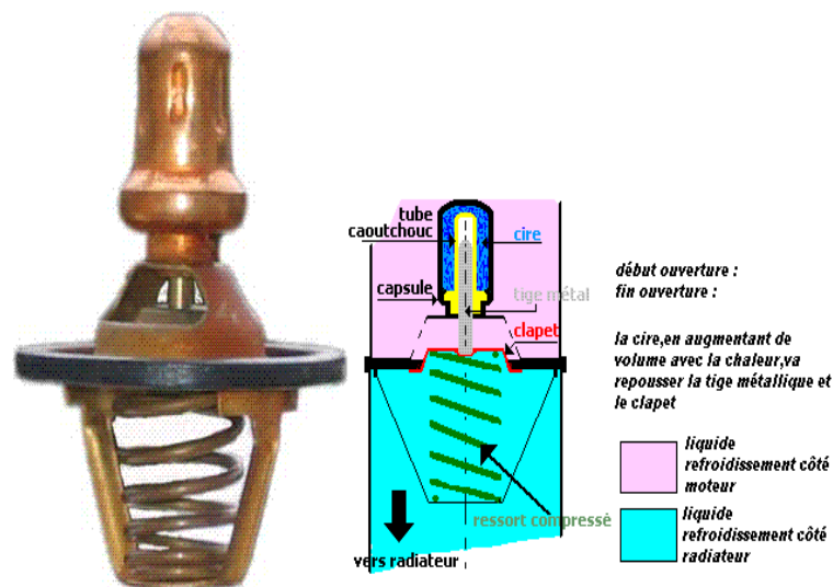
Figure.III.13: thermostat. [9]
