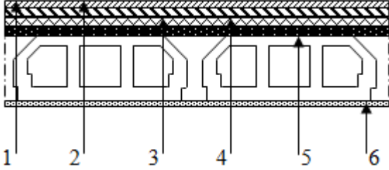
Figure II.3 Terrasse accessible
