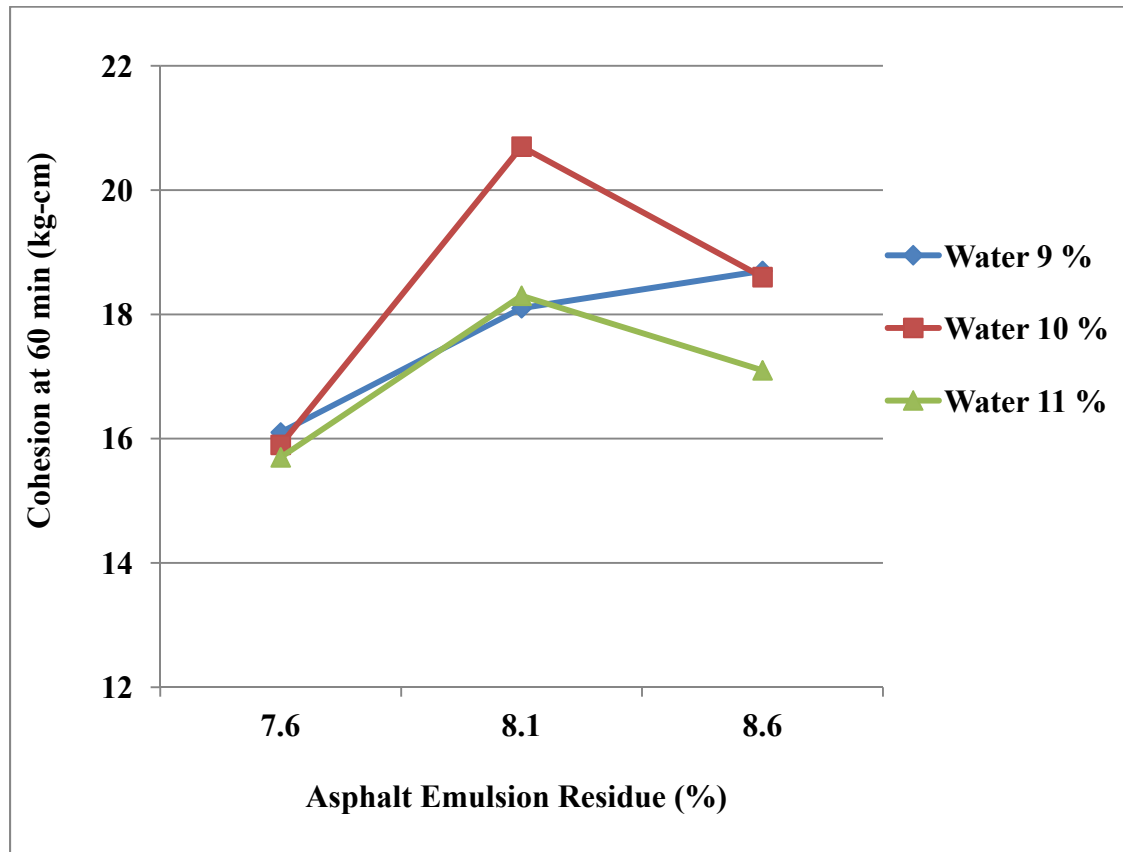
Figure 6.33 60-minute wet cohesion torque values against different asphalt emulsion residue with 9, 10, and 11% water, mixtures prepared with 1% Portland cement
