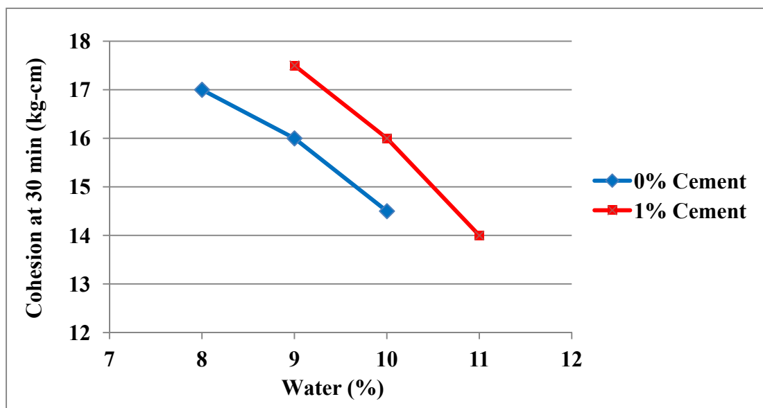
Figure 6.28 Comparison between 30-min cohesion values of mixture prepared with and without Portland cement at 8.6% asphalt emulsion residue
