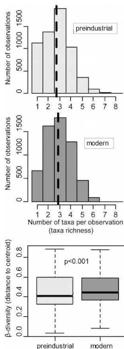
Figure 4.2 Histograms of taxa richness (dashed lines represent mean number of taxa per observation) and \beta -diversity (i.e. multivariate dispersion) for each time period.
