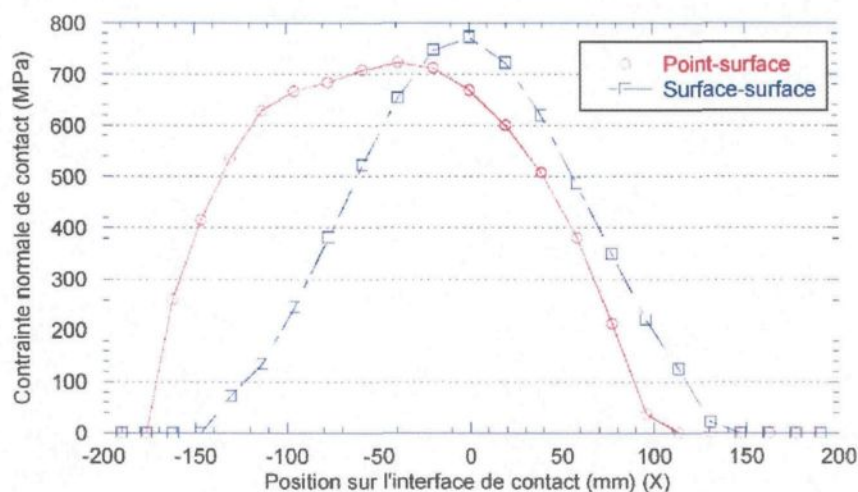
Figure 5.12 – Contrainte normale de contact (maillage 2)
