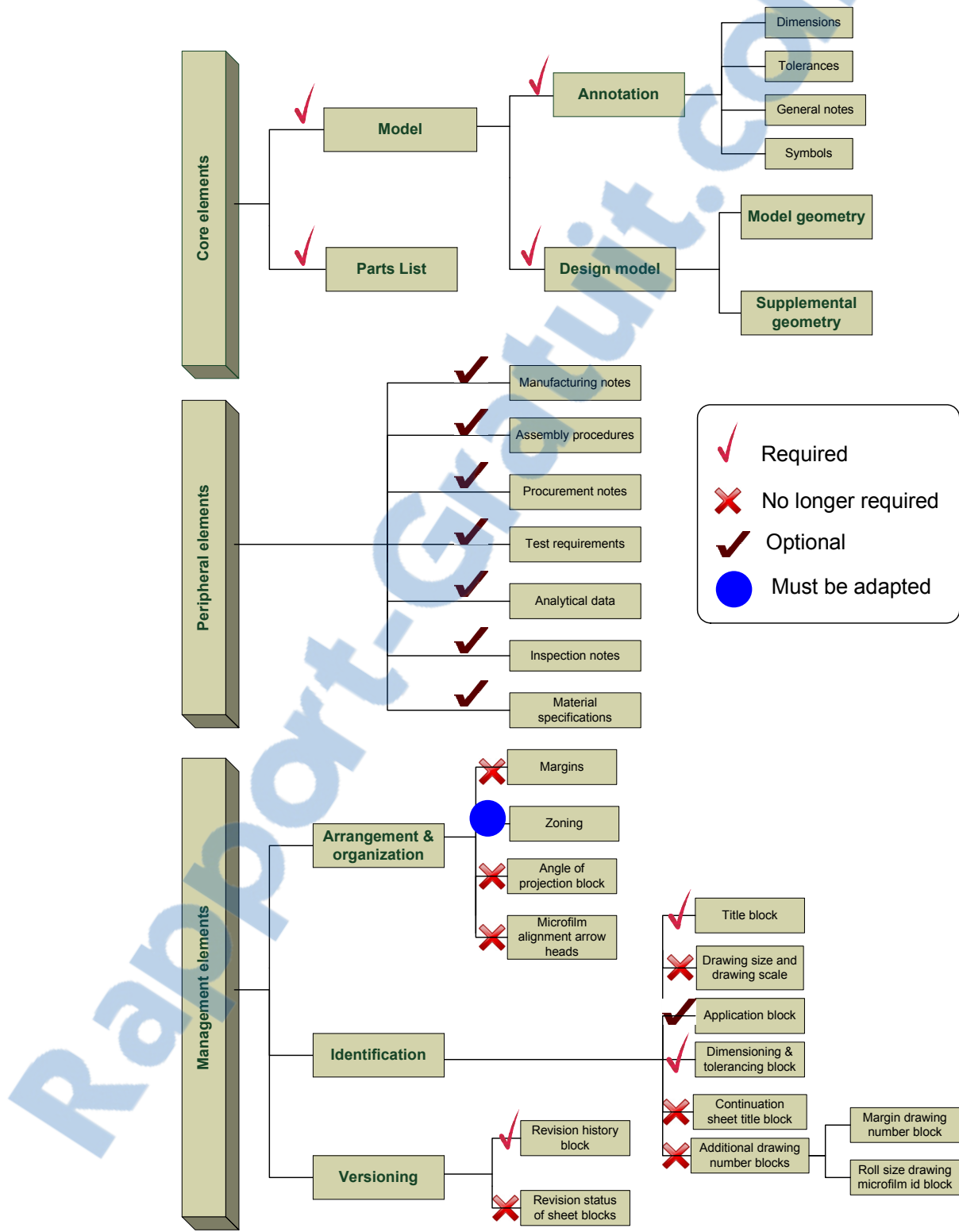
Fig. 3. Drawing elements: classification and transfer to MBD
