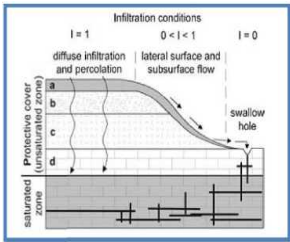
Figure III.1 : Illustration de la méthode PI (Goldscheider, 2005 in Fellah 2012)
