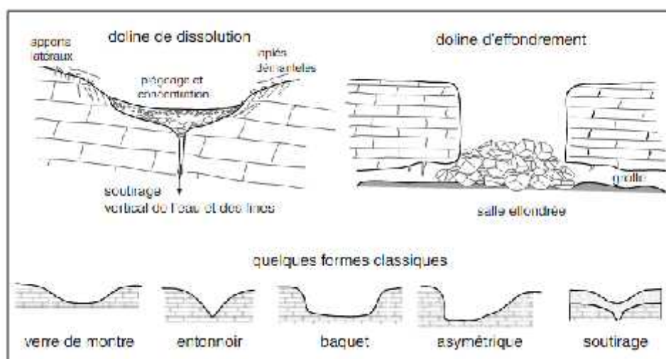
Figure II.2 : Structure des dolines (Gilli, 2011)
