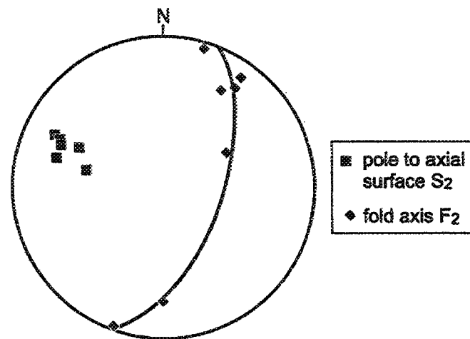
Figure 2.3: Lower hemisphere projection of structural elements for regional folds.
