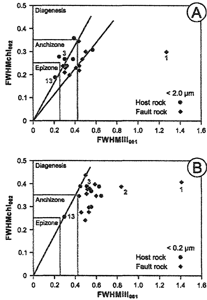
Figure 1.9: Diagram illustrating the variations in the illite crystallinity index (ICI) versus the chlorite crystallinity index (CCI) for A) < 2 \mu\text{m} and B) < 0.2 \mu\text{m} size fractions.
