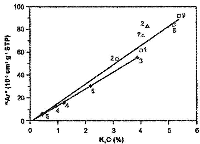
Figure 2.8: K 2 O versus radiogenic 40 Ar diagram for the studied size fractions of the samples from the St-Laurent, Anse-aux-Vaches and Montmorency faults.
