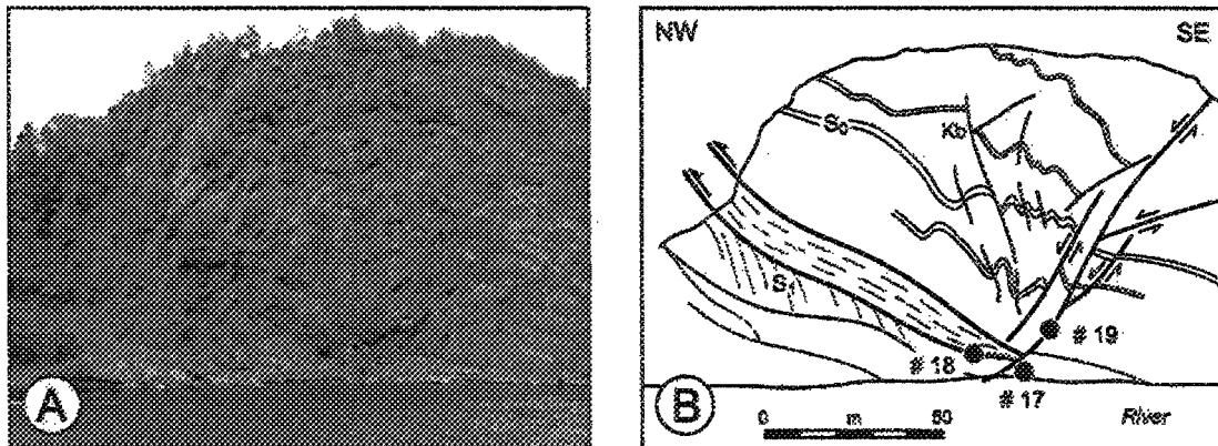
Figure 1.6: Field photograph and sketch of Outcrop H (see Fig. 1.3) showing NW-verging D_2 thrust faults truncated by a NW-dipping D_3 normal fault along the Rivière-du-Loup transect. S_0 = bedding plane; S_1 = foliation; Kb = kink band; # = sample sites (see Tables 1.2 and 1.5).
