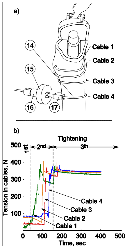
Fig 3: a) Tensioning device and load washer assembly; b) Three-step cable installation procedure: 1) positioning; 2) initial tightening; 3) retightening.
