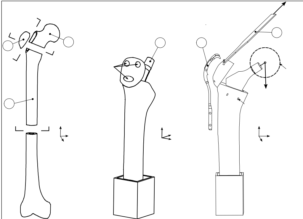
Fig 1: Specimen preparation: a) cuts of the femoral model; b) implantation of the femoral prosthesis; c) implantation of the abductor force application strap and simulated physiological forces P1, P2 (arrows).
