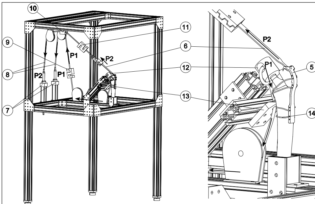
Fig 2: Test bench.
