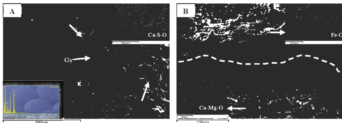
Figure 3.4 SEM-EDS images of the surface of dolomite from D20 (dol-D20) and D80 (dol-D80) after the treatment: (A) Surface of dol-D20 covered by gypsum (Gy) and Fe-oxyhydroxides, (B) Layer of ~50µm of precipitates (srebrodolskite, portlandite) and Fe-oxyhydroxides on the surface of the dol-D80
