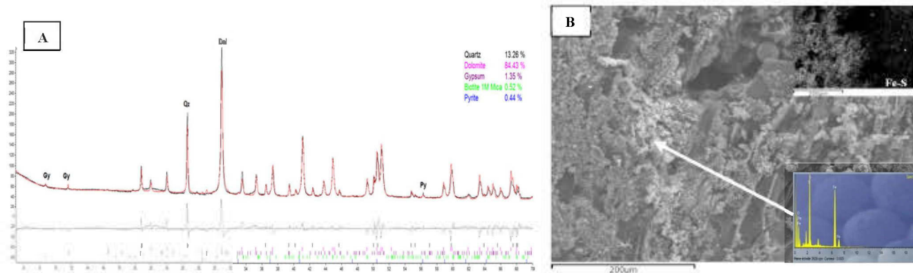
Figure A.2 (A) Diffractogram showing the presence of gypsum and pyrite as the secondary crystallized minerals in D50, (B) SEM-EDS images of Fe-oxyhydroxides and pyrite on the surface of wood chips in WA80
