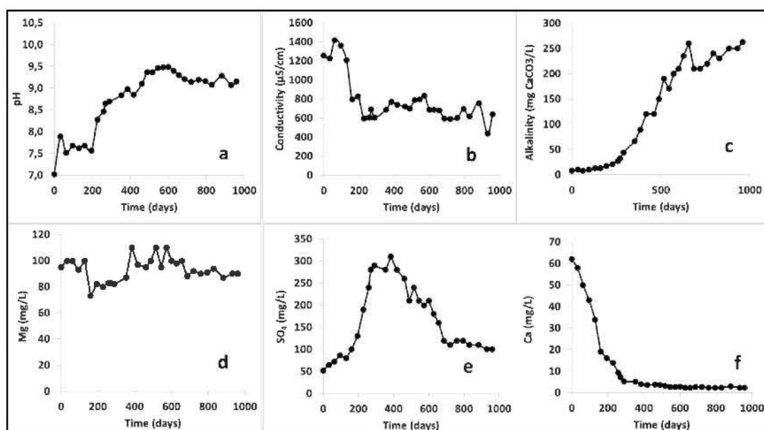
Figure 2.1 Geochemistry of leachates from column: pH (a), Conductivity (b), Alkalinity (c), Mg (d), \text{SO}_4 (e), and Ca (f)
