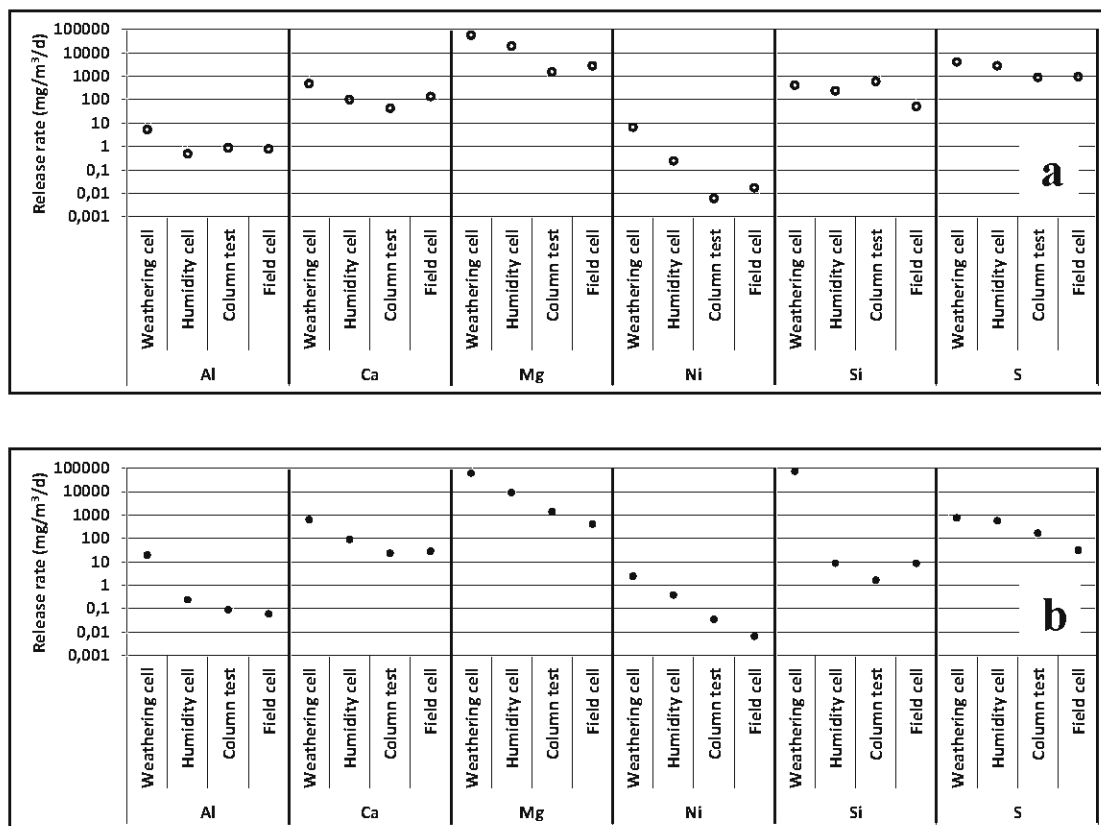
Figure 4.4 Volume-normalized release rate ( \text{mg}/\text{m}^3/\text{d} ) for selected elements for tailings (a) and waste rock (b); log scale
