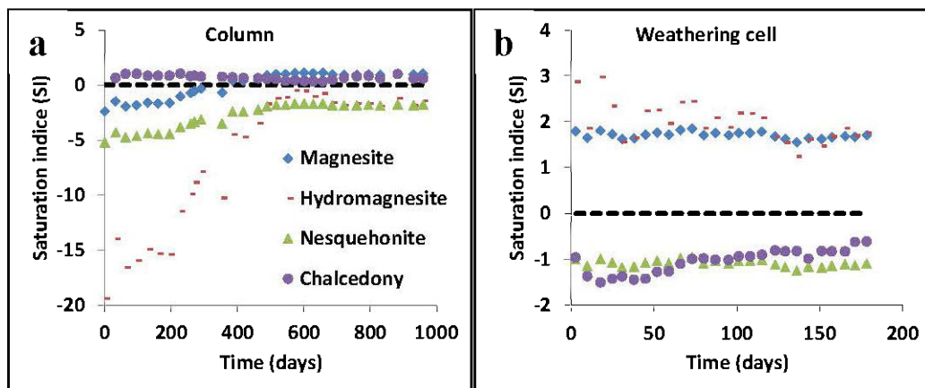
Figure 2.5 Saturation indices evolution calculated with Visual Minteq for tailings column (a) and weathering cell leachates (b); dashed line represent the equilibrium point
