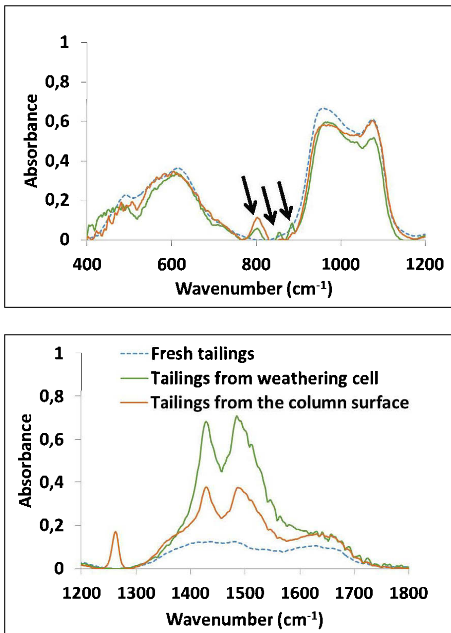
Figure 2.10 DRIFT results for fresh and weathered tailings: (a) 400\text{-}1200\text{ cm}^{-1} ; (b) 1200\text{-}1900\text{ cm}^{-1}
