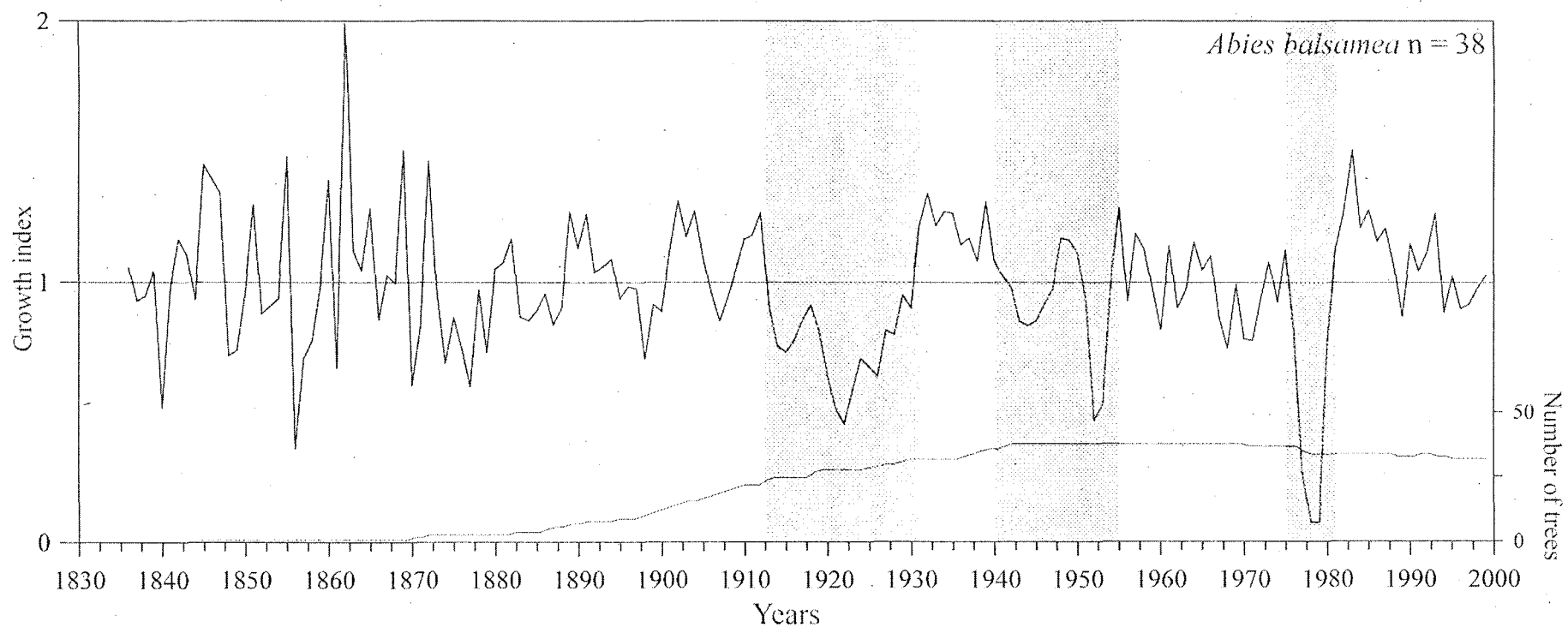
Figure 2.5 Standardized tree-ring chronology of balsam fir ( Abies balsamea ) trees sampled in the PLT study site. The shaded areas represent spruce budworm outbreaks that affected the study area.
