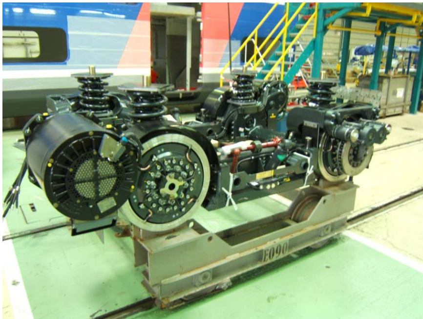
Figure 7: Bogie moteur
