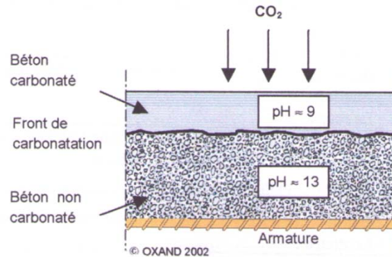
Figure 1. 13 Progression de la carbonatation (Oxand, 2002)
