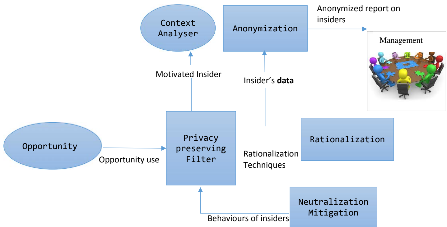
Figure 5.7 Privacy-preserving filter
