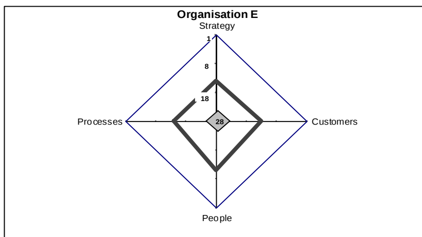
Figure 5.3: Radar diagram illustrating strategic alignment for organisation E
