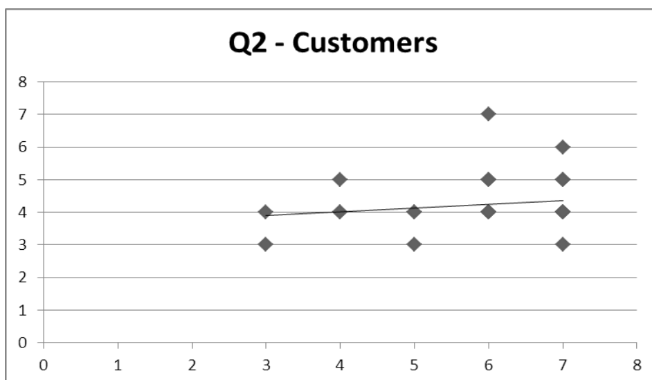
Figure 4.8: Scatterplot depicting Q2 – customers
