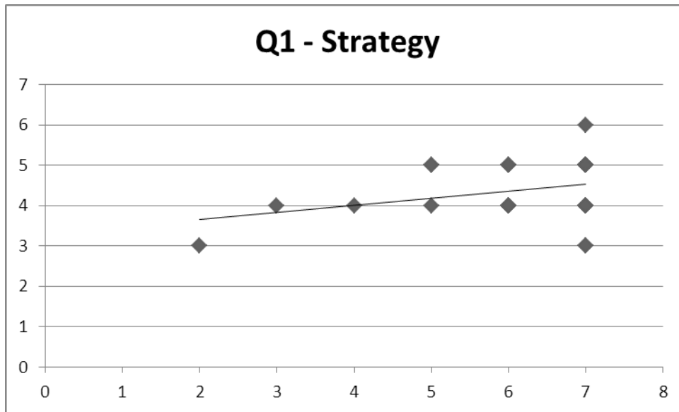
Figure 4.7: Scatterplot depicting Q1 – strategy
