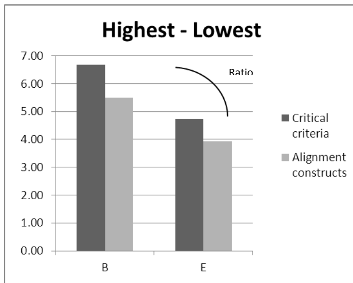
Figure 5.1: Graphical representation of the highest and lowest organisational scores for the two variables
