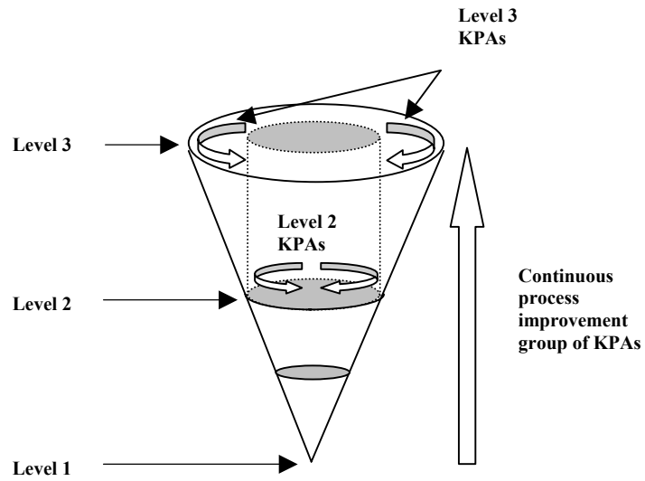
Figure 10.2: Maturity level 3
