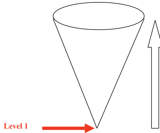
Figure 3: Maturity level 1
