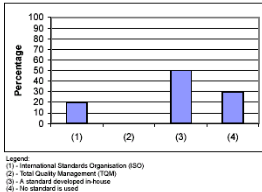
Figure 4.6: Standards used
