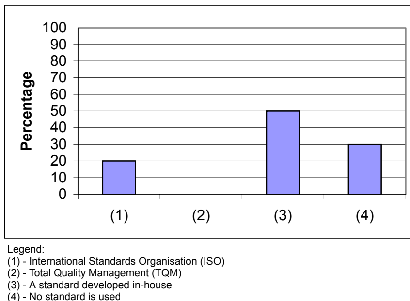
Figure 5. Standards used.
