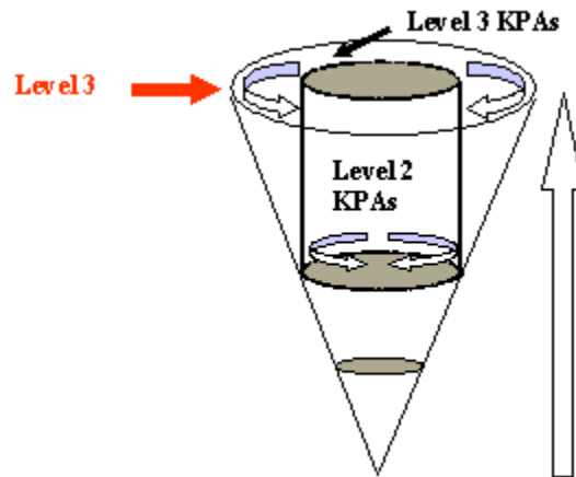
Figure 7.8: Maturity level 3
