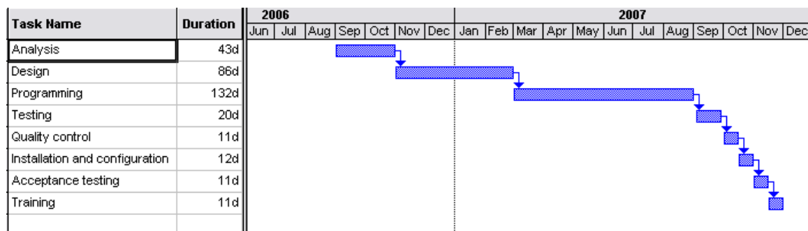
Figure 12.3: Project schedule
