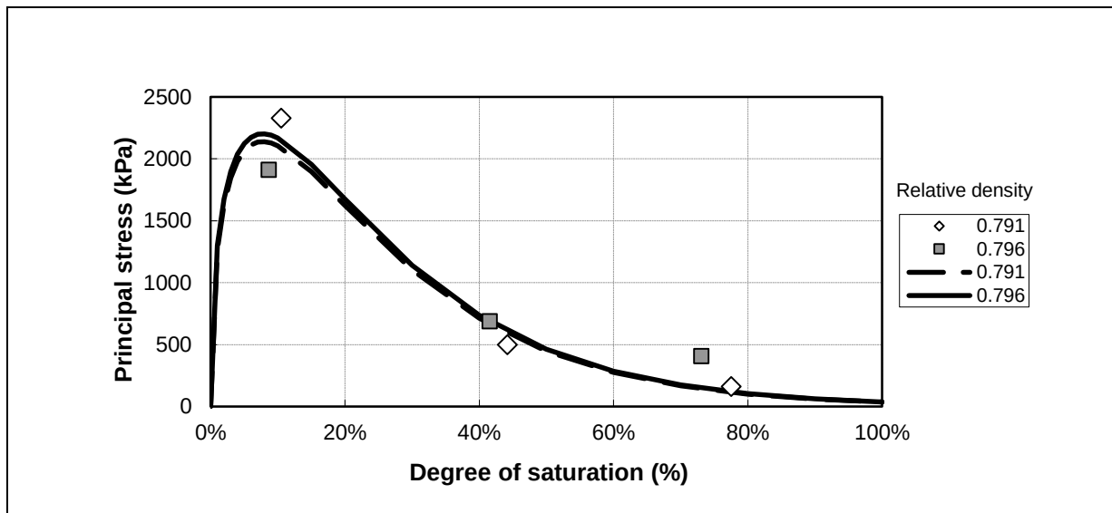
Figure D.6: Suction model and measured stress at zero confinement pressure for Road S191 base layer.
