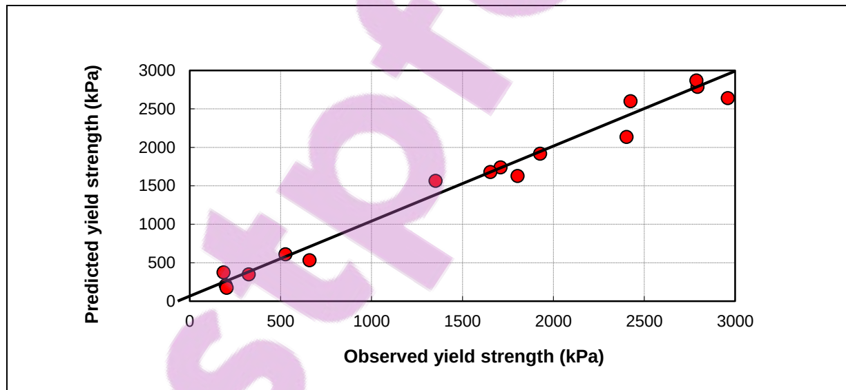
Figure D.1: Failure stress plot for N4 extension base layer.
