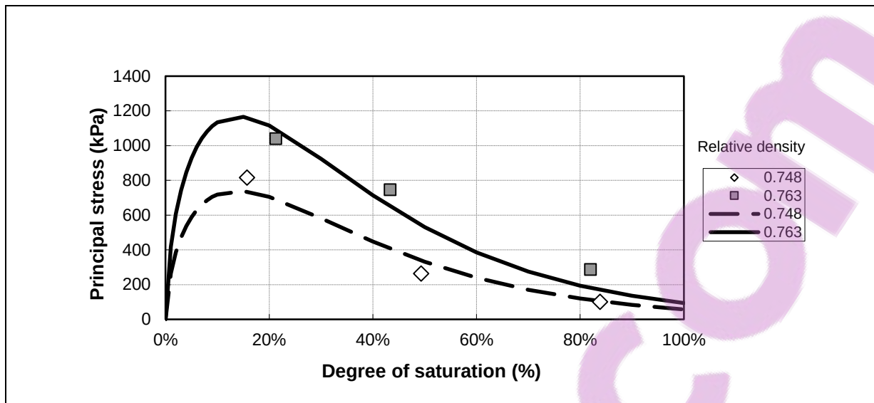
Figure D.8: Suction model and measured stress at zero confinement pressure for Road P10-2 base layer.
