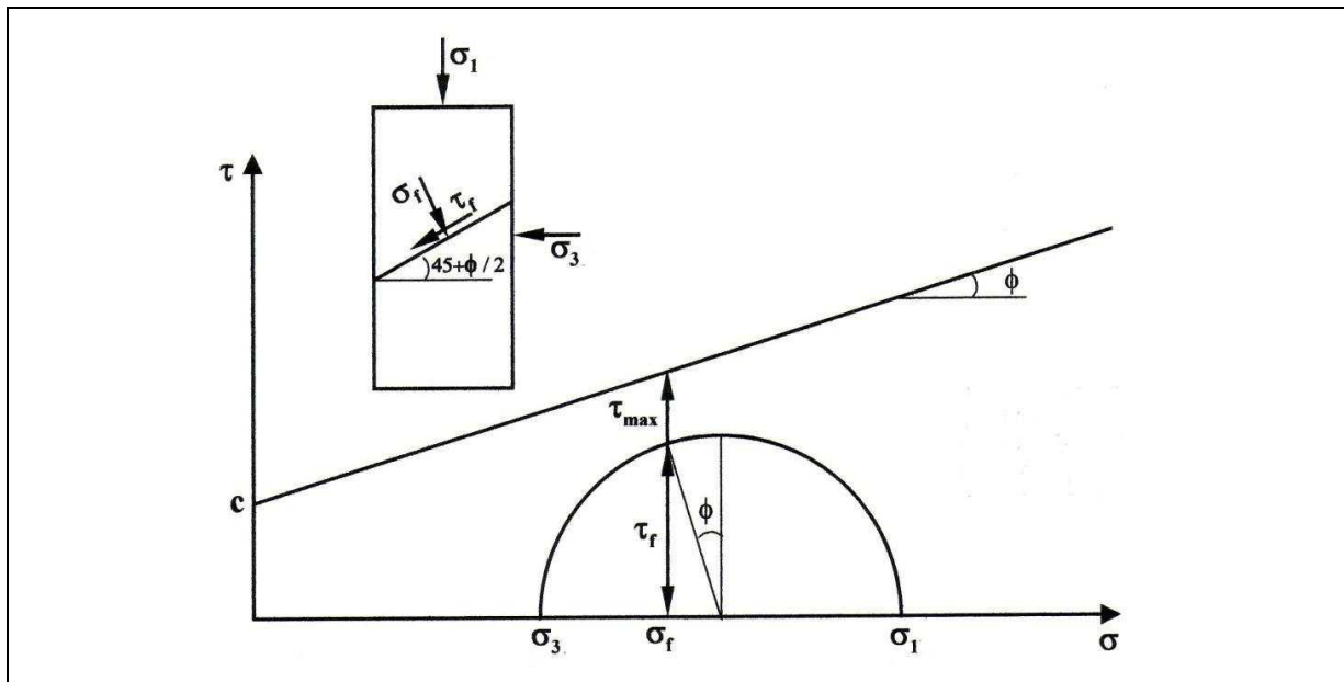
Figure B.3: Mohr-Coulomb representation of shear strength and applied stress states (Anochie-Boateng, 2007).
