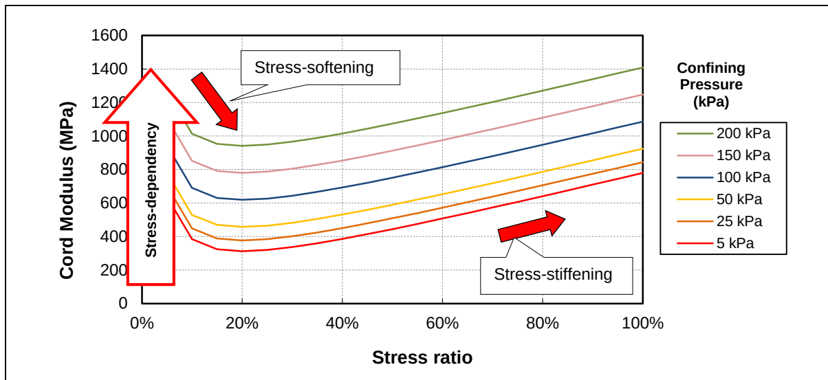
Figure 4.17: Stress-dependent behaviour of material.
