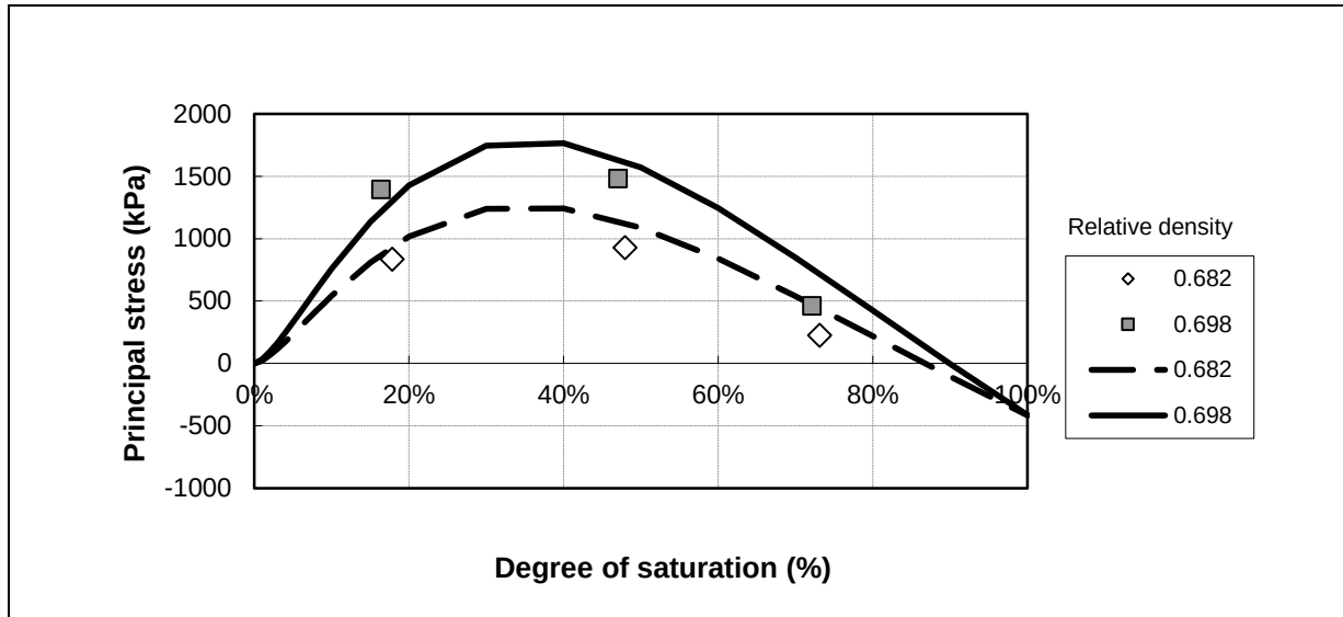
Figure D.4: Suction model and measured stress at zero confinement pressure for N4 extension upper selected layer.
