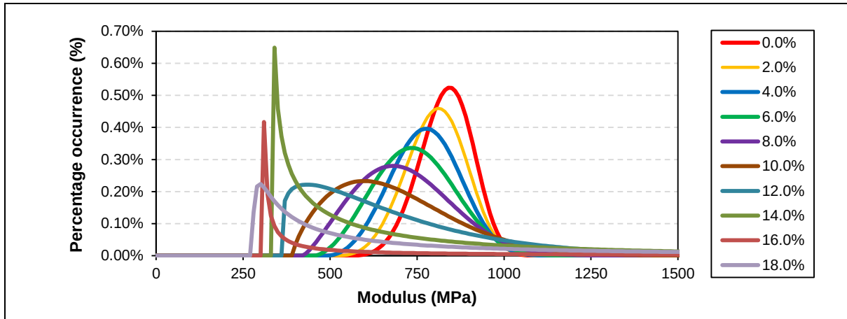
Figure 5.25: Family of Weibull (3P) distributions for Sample 11727 data.
