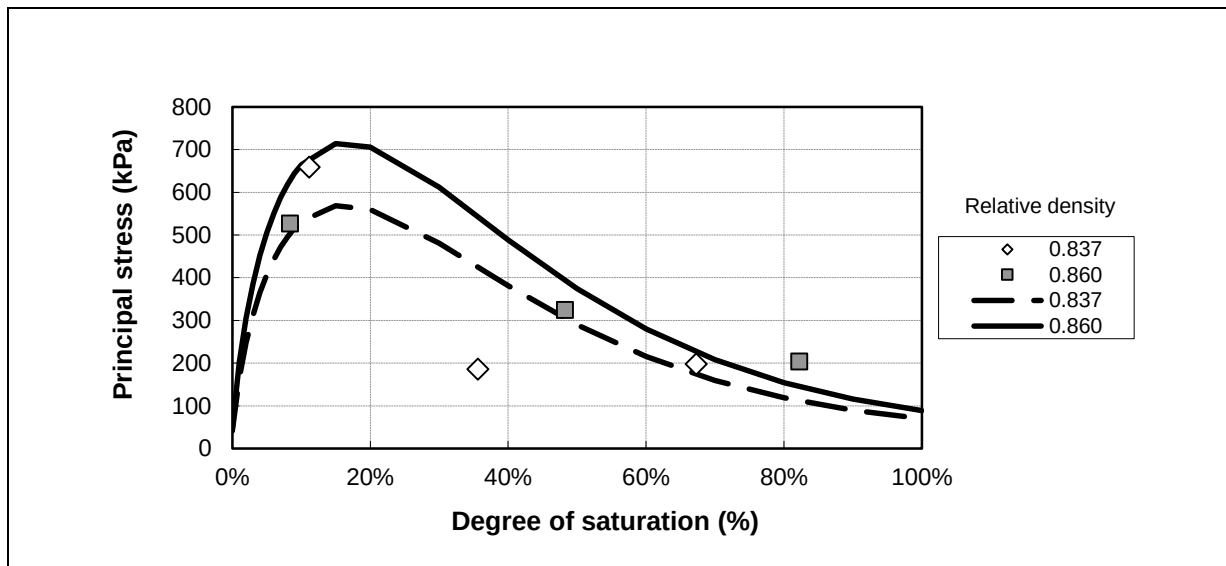
Figure D.2: Suction model and measured stress at zero confinement pressure for N4 extension base layer.
