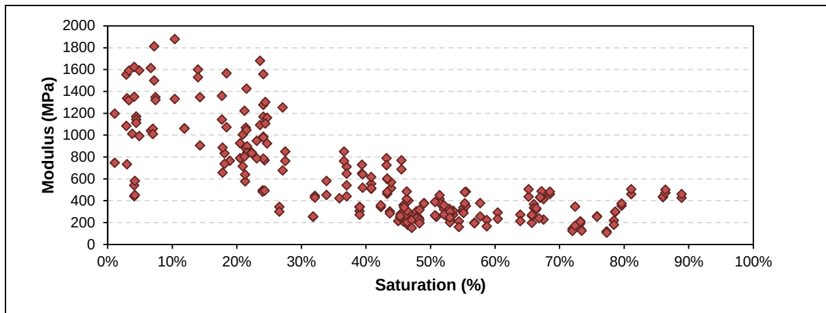
Figure 5.22: Modulus versus saturation relationship for data published by Theyse (2008a).
