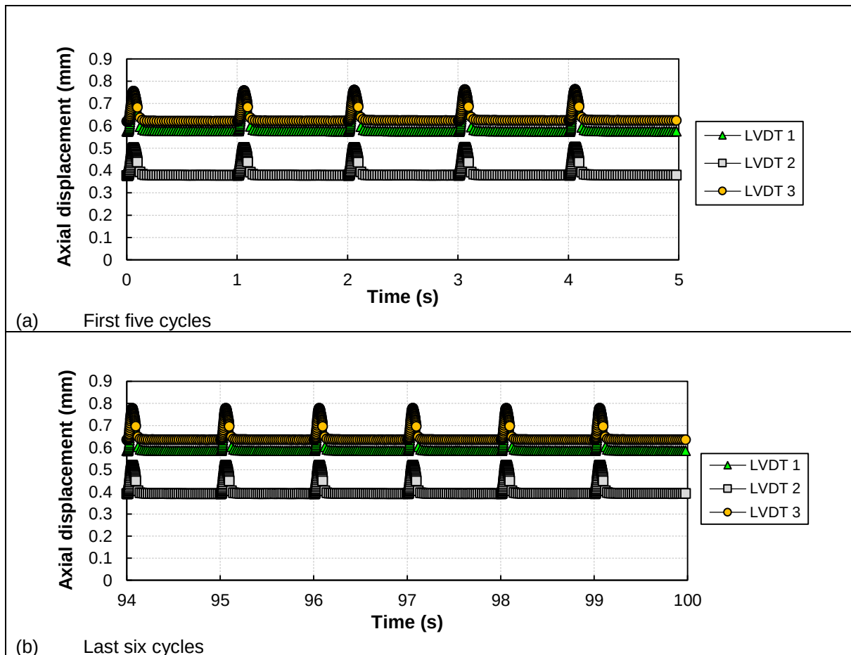
Figure 4.10: Axial displacement recorded during a 100 load cycle for D804 B (Sample no. 11728-28).
