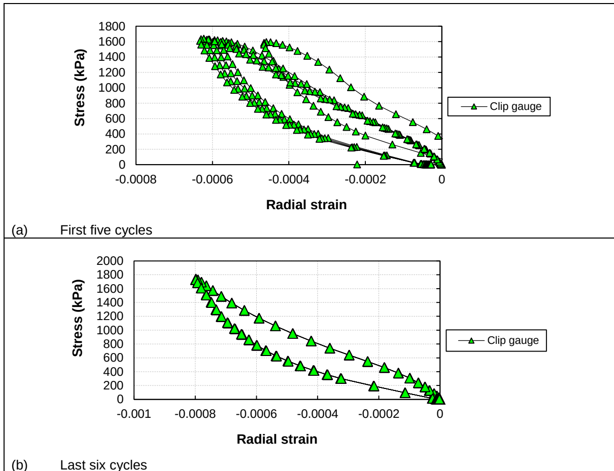
Figure 4.13: Circumferential load-displacement hysteresis loops recorded during a 100 load cycle sequence for D804 B (Sample no. 11728-28).
