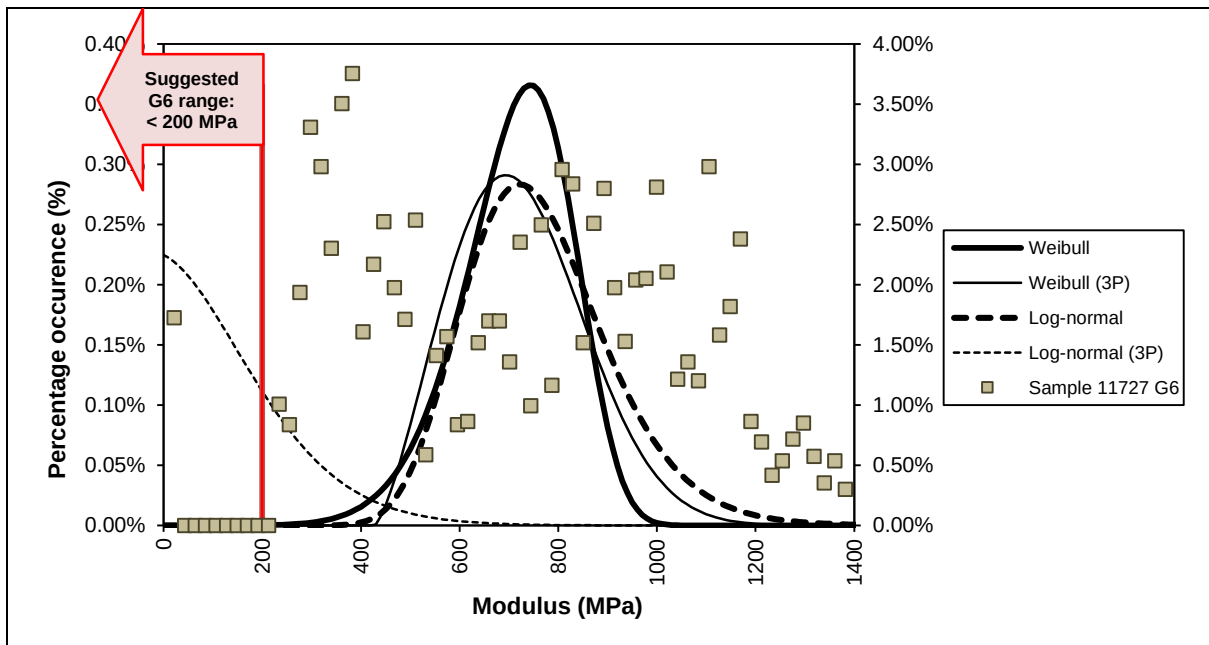
Figure 5.24: Predictive statistical distributions and suggested range for Sample 11727 data.
