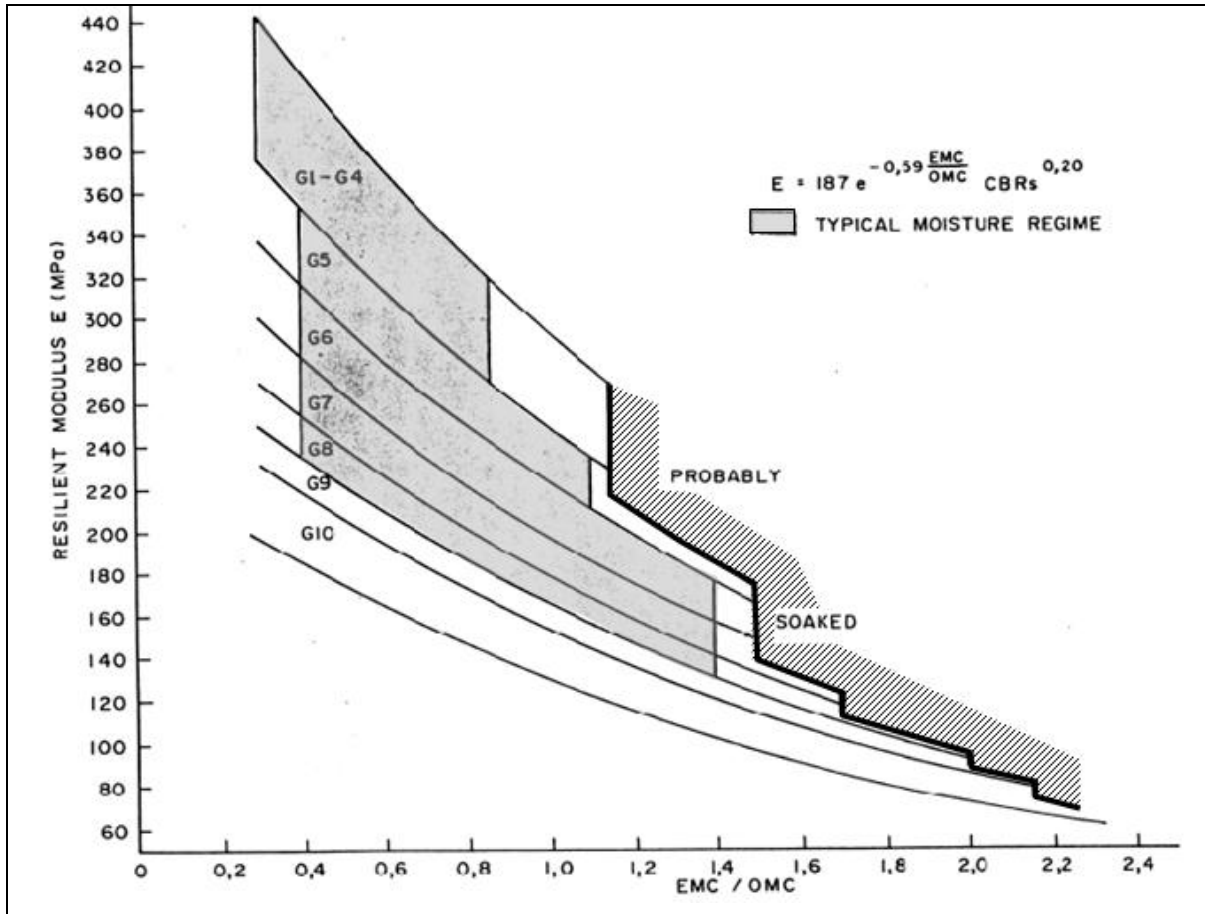
Figure 2.17: Variation of resilient modulus with moisture for material classes G1 to G10 (Emery, 1985).
