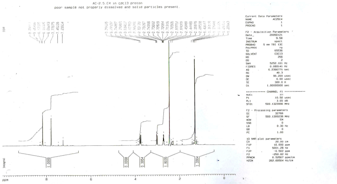
Figure 2.9: 1 H-NMR spectrum of indane.
