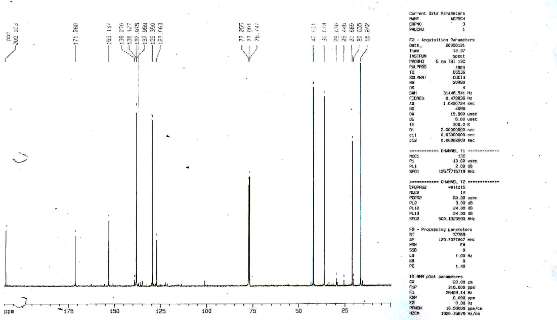
Figure 2.10: 13 C-NMR spectrum of indane.
