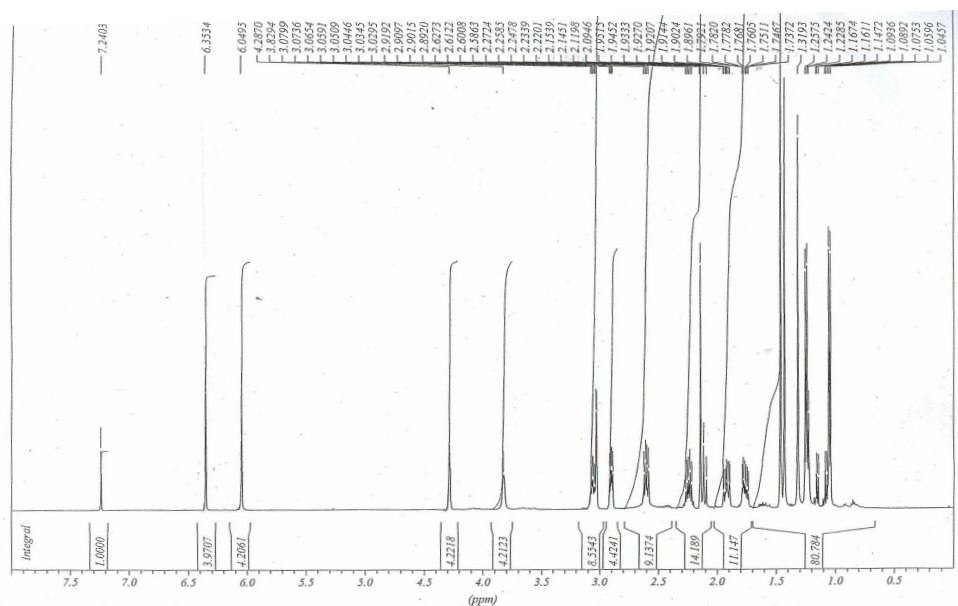
Figure 2.23: 1 H-NMR spectrum of steenkrotin B.
