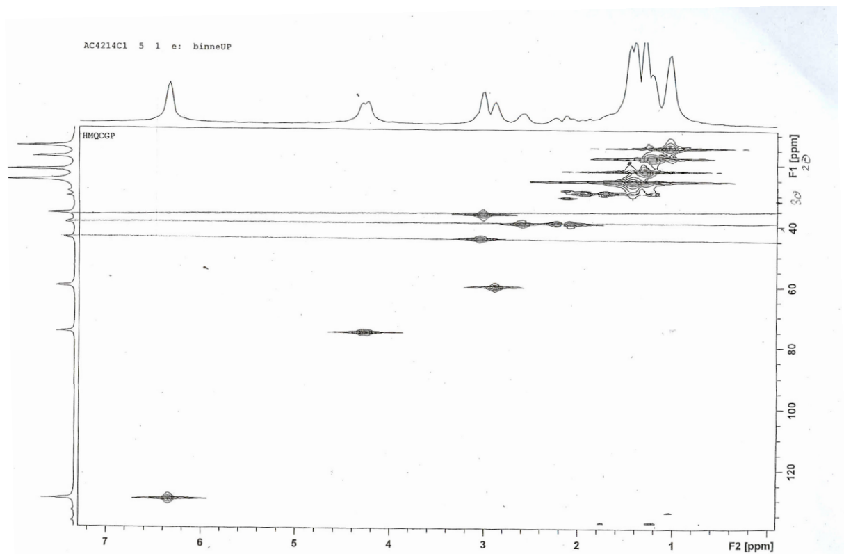
Figure 2.27: HMQC spectrum of steenkroton B.
