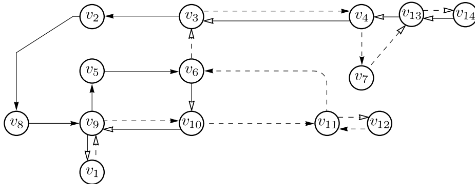
(c) With the introduction of the intermediate facility a single vehicle can now service the complete area. The complete route is [1, 9, 10, 11, 12, 11, 6, 3, 4, 7, 13, \mathbf{14}, 13, 4, 3, 2, 8, 9, 5, 6, 10, 9, \mathbf{1}] . Visits to intermediate facilities at v_{14} and v_1 are shown in bold. The total waste collected with the dashed subroute ( v_1 to v_{14} ) and the solid subroute ( v_{14} to v_1 ) are 23 kg and 20 kg, respectively, and the total distance of the route is 520 meters. A solid arrow-head indicates that a vehicle services that edge or arc, and an empty arrow-head indicates that a vehicle only traverses it.
