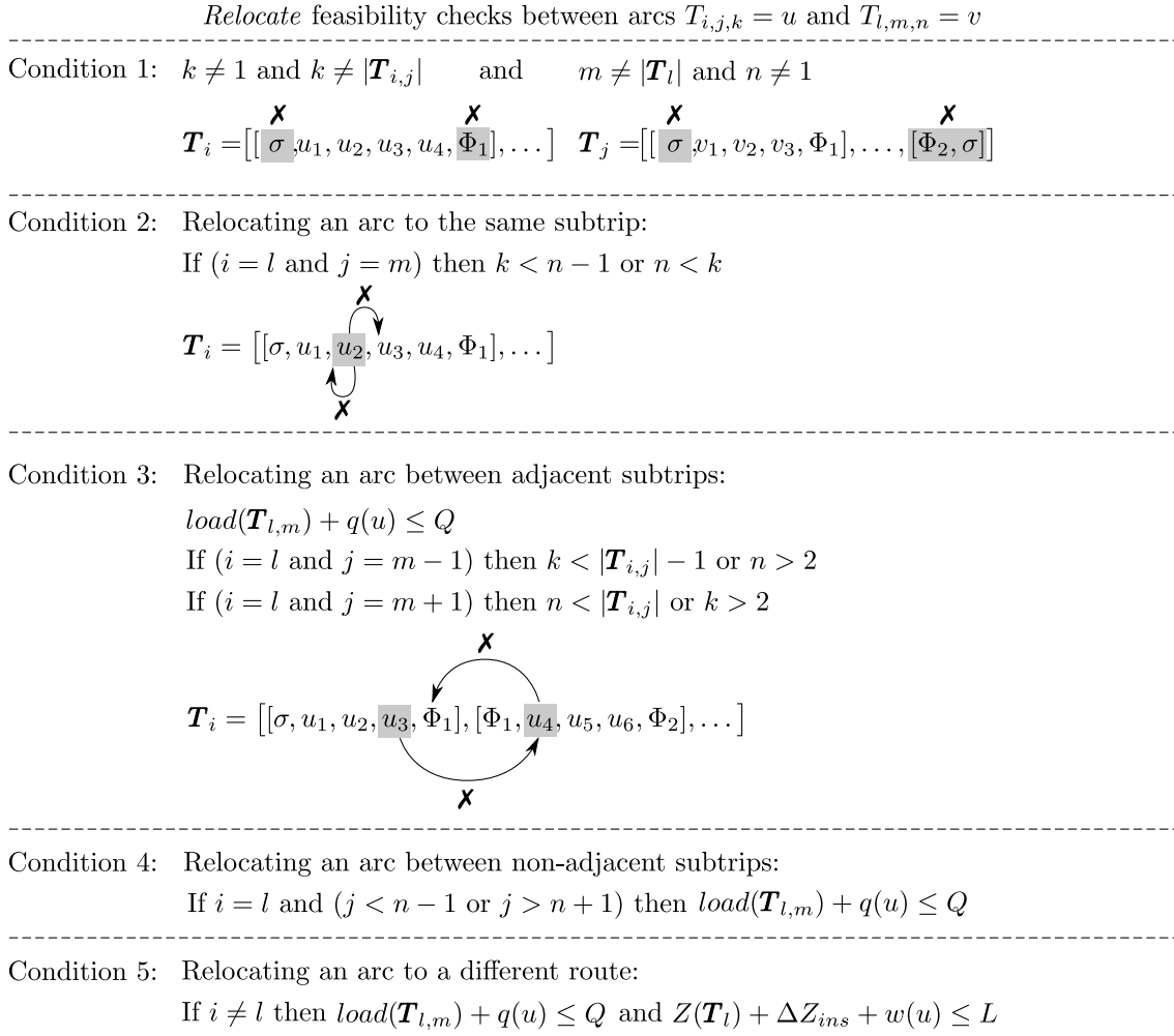
Figure 5.7: Conditions for relocating arc T_{i,j,k} to position T_{l,m,n} .
