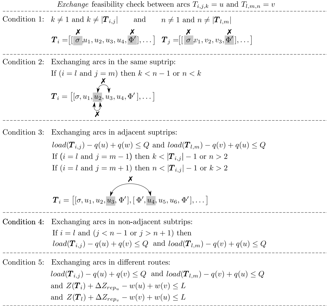
Figure 5.10: Conditions for exchanging arcs T_{i,j,k} and T_{l,m,n} .
