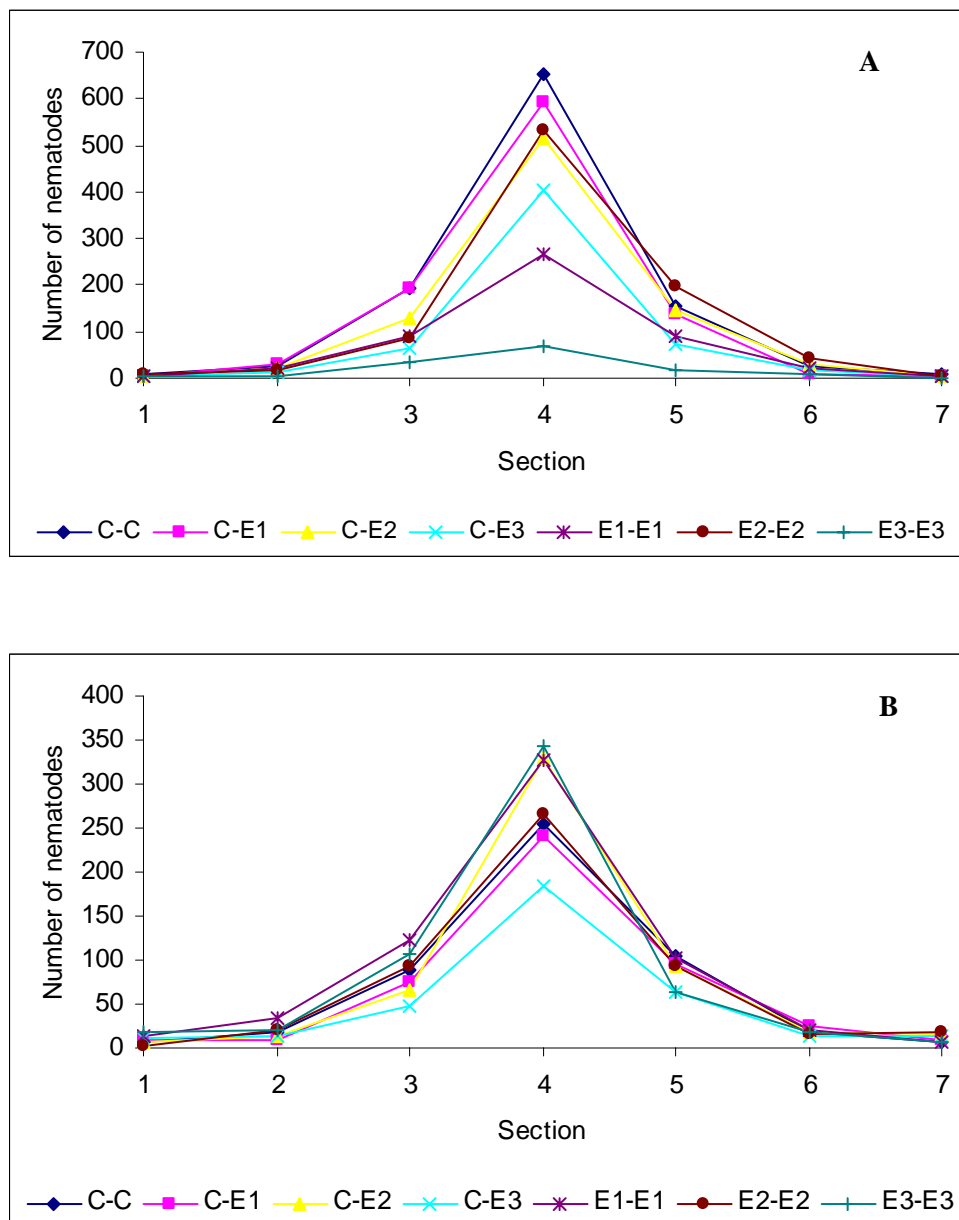
Figure 8: Distribution of nematodes in the polyvinyl chloride (PVC) sections showing migration of nematodes towards endophyte-inoculated and un-inoculated banana plants paired in a PVC tube apparatus divided into seven sections (A, bioassay 1; B, bioassay 2). Radopholus similis (2000 mixed stages) were introduced in the middle section of the PVC apparatus (section 4) equal distances from both plants placed in sections 1 and 7, which contained either an endophyte-inoculated or un-inoculated plant.
