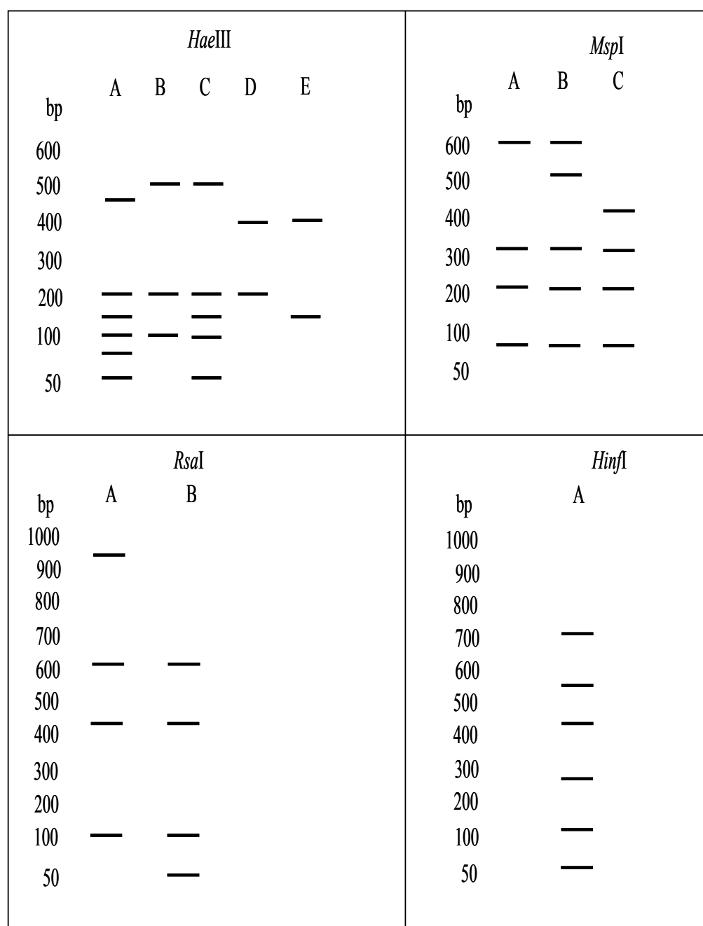
Figure 1. Schematic representation of PCR-restriction fragment length polymorphism patterns after digestion of the intergenic spacer region of the ribosomal DNA of 46 isolates of endophytic Fusarium oxysporum with the restriction enzymes Hae III, Msp I, Rsa I and Hinf I.
