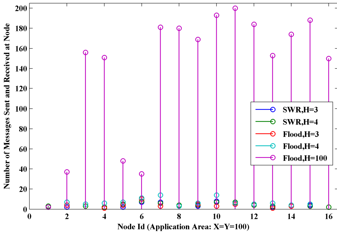
Figure 5.9: SWR and flooding (not restricting flooding hop count where 100 hops is equivalent to no restriction)
