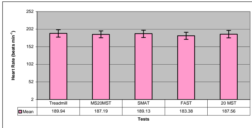
Figure 4.4: Mean Maximal Heart Rate (beats min -1 ) Comparison Between Tests (n=16)
