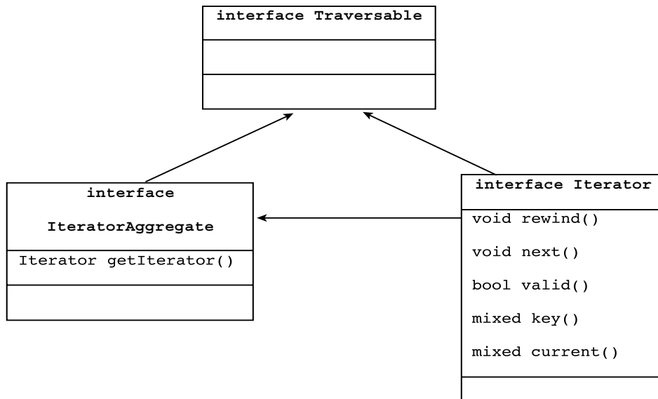
Fig. 4.2 Class diagram of Iterator hierarchy.
