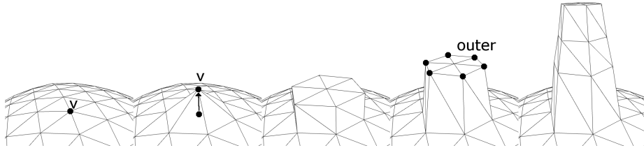
Figure 4: A sequence generated by applying the new_spike operation in Listing 2 to vertex v . The sequence alternates between moving the vertex (and its neighbours) and inserting a new set of faces on the end of the protrusion. The variable outer in Listing 3 refers to the vertices at the end of the cap (as shown).
