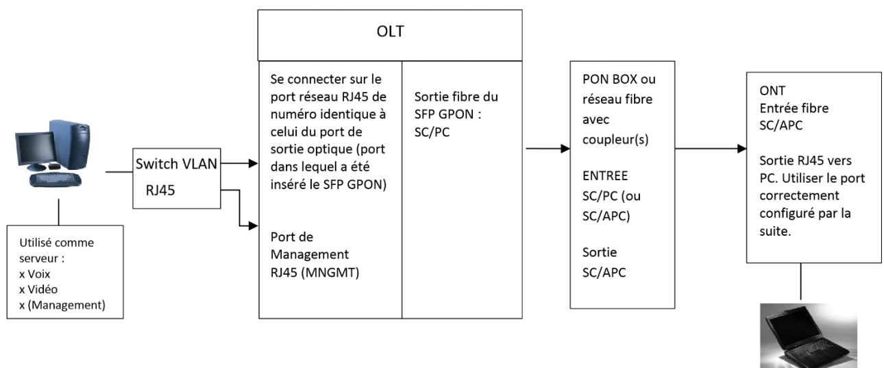
Figure 7 installation triple-play
