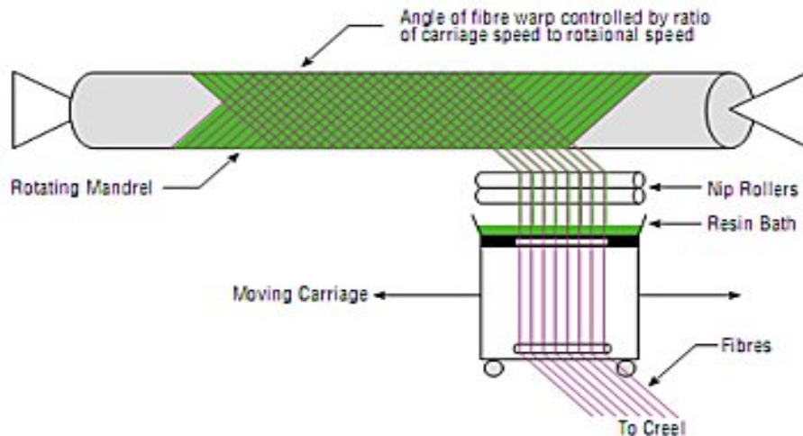
Figure 2.7 Filament winding
