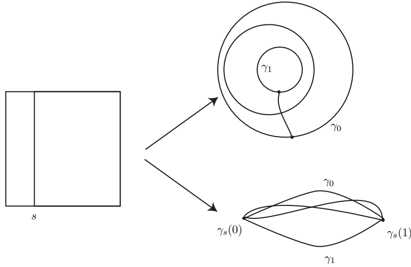
FIGURE 4. Homotopies
