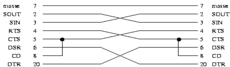
Illustration 9: Câble NULL-MODEM complet
