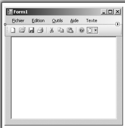
Figure 6.11 : ToolStrip standard
