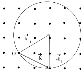
Figure 8.17: Construction d'Ewald.
