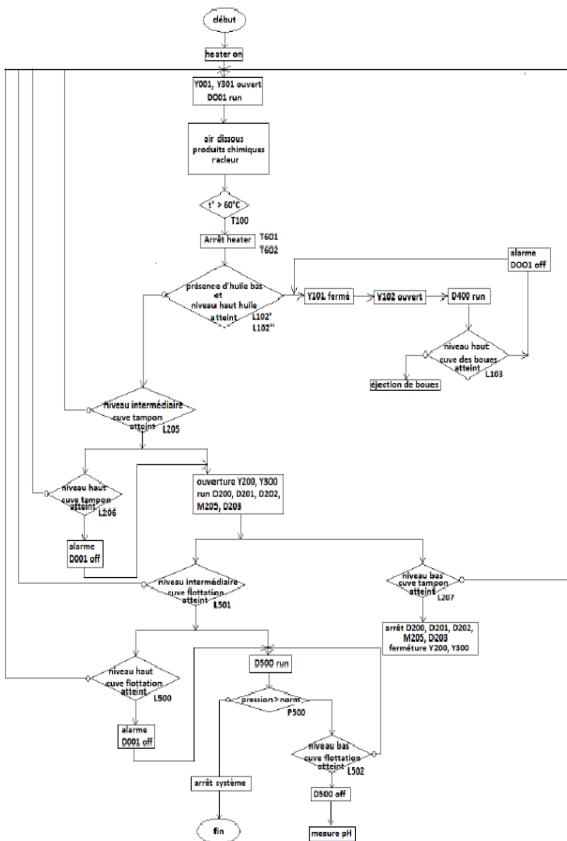
Figure 41: système principal
